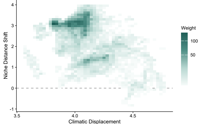
(a) Climatic Displacement vs Niche Distance Shift
