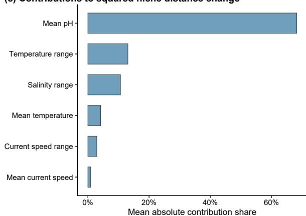
(c) Contributions to squared niche distance change
