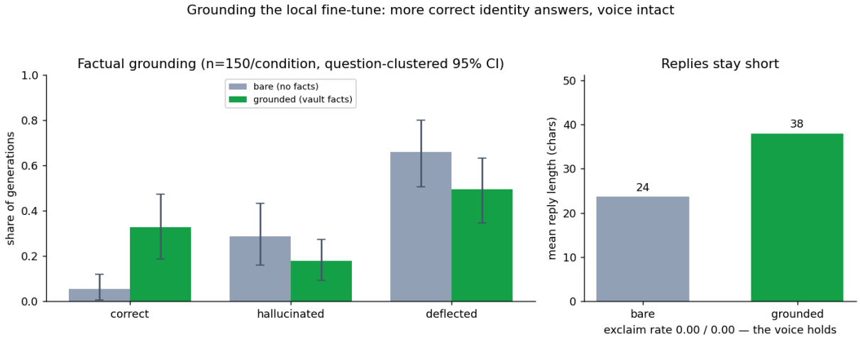
Figure 14: Bare vs grounded local fine-tune, n = 150 generations per condition. Left: grounding lifts the correct-fact rate from 0.05 to 0.33 (question-clustered 95% intervals disjoint) and lowers hallucination from 0.29 to 0.18 (intervals overlap — a directional drop). Right: replies stay short (24 → 38 characters) and the “!” rate stays at 0.00 — the card adds facts without moving the voice.
