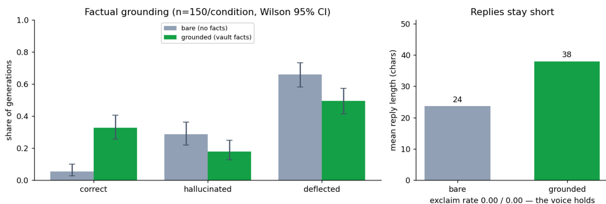
Figure 14: Bare vs grounded local fine-tune, n = 150 generations per condition. Left: grounding lifts the correct-fact rate from 0.05 to 0.33 (Wilson 95% intervals disjoint) and lowers hallucination from 0.29 to 0.18 (intervals overlap — a directional drop). Right: replies stay short (24 \rightarrow 38 characters) and the “!” rate stays at 0.00 — the card adds facts without moving the voice.
