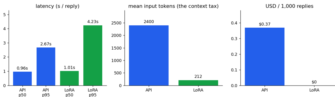
Figure 13: Operational profile (Arm A). The LoRA is free and lean; the API pays a \sim 11\times input-token tax and a per-call fee to reach the fine-tune’s fidelity.
