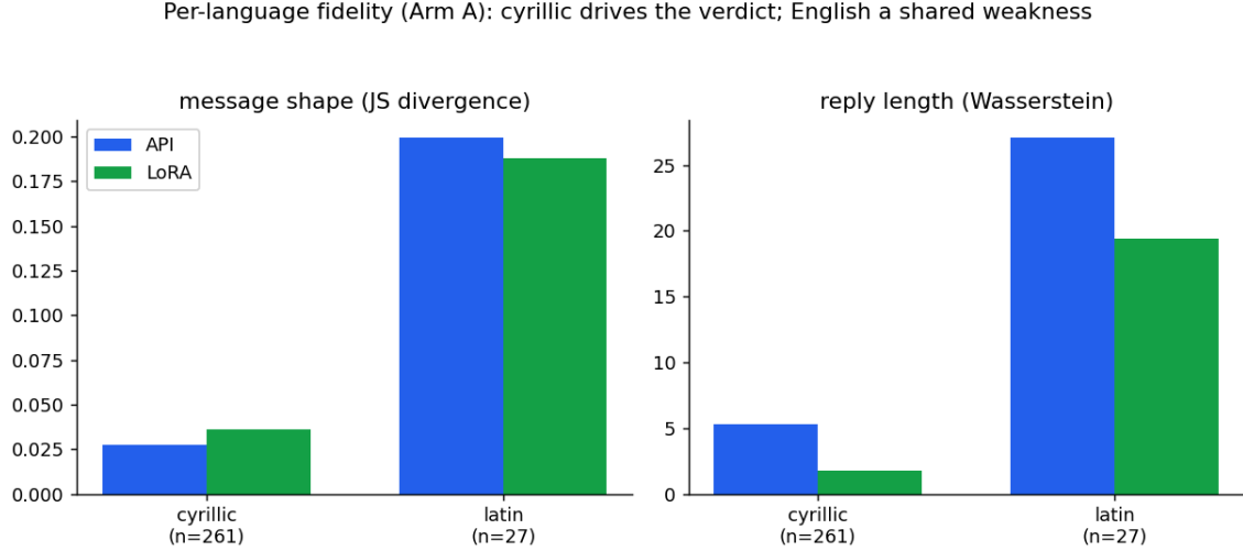
Figure 10: Per-language fidelity (Arm A). Cyrillic ( n = 261 ) drives the verdict; English ( n = 27 ) is a tie and a shared weakness for both backends.
