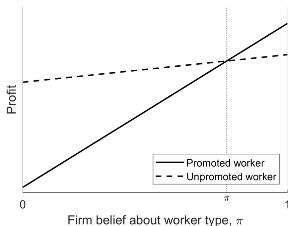
Figure 3.1: Expected Profit as Function of \pi, p
