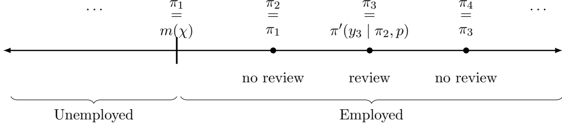
Figure 3.2: Evolution of \pi
