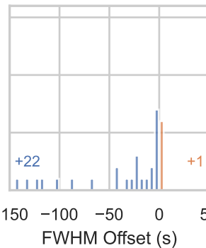
Transformer, Loose
