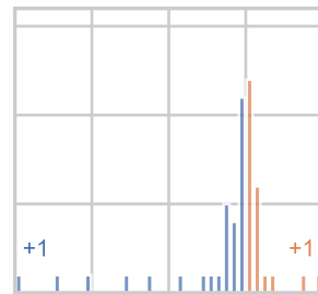
Transformer, Tight
