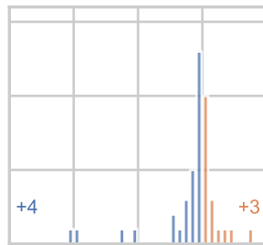
LSTM, Tight
