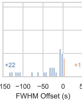
LSTM, Loose
