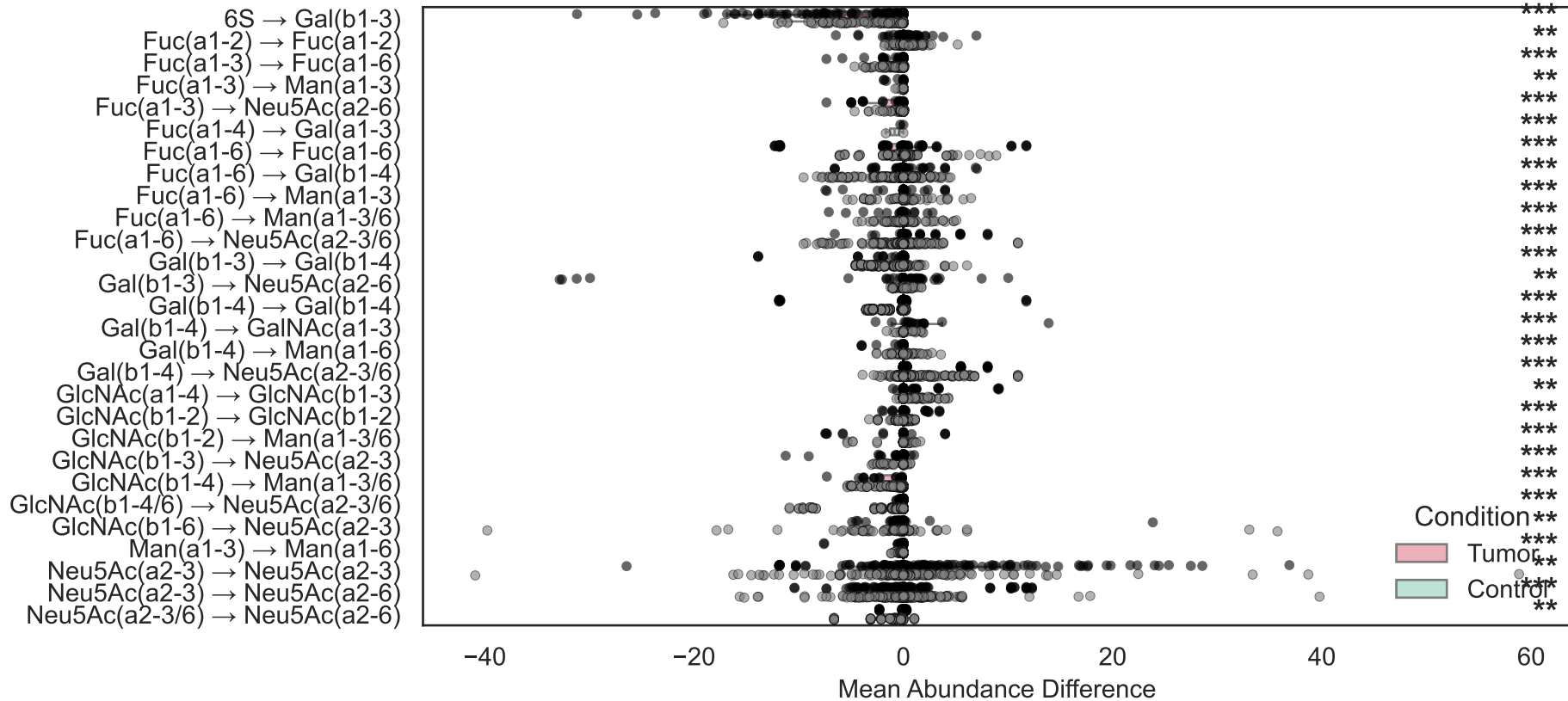
Variance in Mean Abundance Between Additions in Diamond Motifs (Tumor vs Control)
