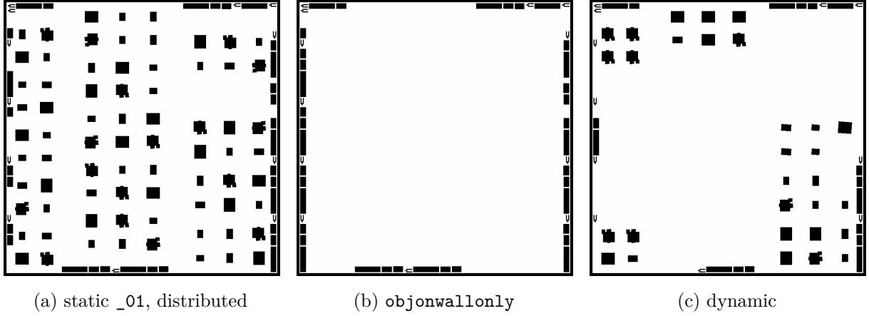
Figure 3.4: Baked occupancy truth of the three large-warehouse object arrangements, each 42.2m square at 0.05 m per cell with origin (-21.1, -21.1) m. Black is occupied, white is free; there is no unknown space because the grids are rasterised from collision geometry rather than observed. Occupied cells are 17.79 % of (a), 8.74 % of (b) and 10.98 % of (c). Panel (b) clears the central floor and keeps obstacles against the walls, which is the arrangement used by dataset_allsensor_002 and dataset_allsensor_003 . No occupancy grid is shown per floor treatment, and none exists : the bayline and plain floors differ only in surface material, which carries no collision geometry, so their baked grids are identical to the panels above. See figure 3.5 .
