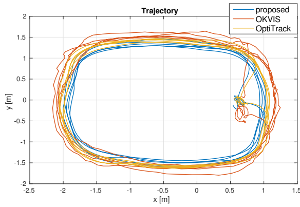
Fig. 10. Trajectory of real world experiment. We hold the sensor and walked five circles. Proposed method compares against OKVIS and OptiTrack.
