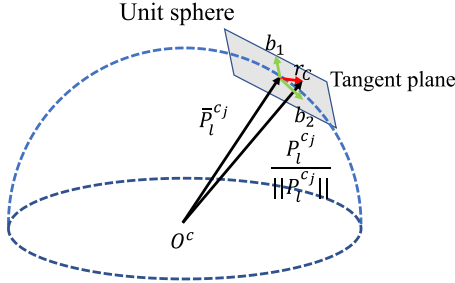
Fig. 6. Illustration of the visual residual on a unit sphere. \hat{P}_l^{c_j} is the unit vector for the observation of the l th feature in the j th frame. P_l^{c_j} is predicted feature measurement on the unit sphere by transforming its first observation in the i th frame to the j th frame. The residual is defined on the tangent plane of \hat{P}_l^{c_j} .
