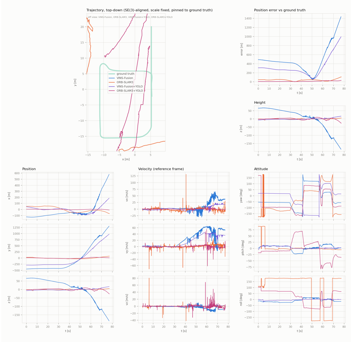
Figure 4.7: Representative repeated-run trajectory diagnostic for dataset_dynamic_nof_loortexture_00_000/logging_20260916_01 , in the same visual format as the existing comparison figures. The table gives the per-system summary for this run; “clean” is ATE RMSE over the longest jump-free segment. The very large paths and frequent jumps are retained rather than clipped into a favourable view. ATE and rotational errors use the rosbag /ground_truth/odometry topic after rigid SE(3) alignment with scale fixed. The nominal VINS+YOLO trace is invalid as a filtering treatment because no masks were matched.
