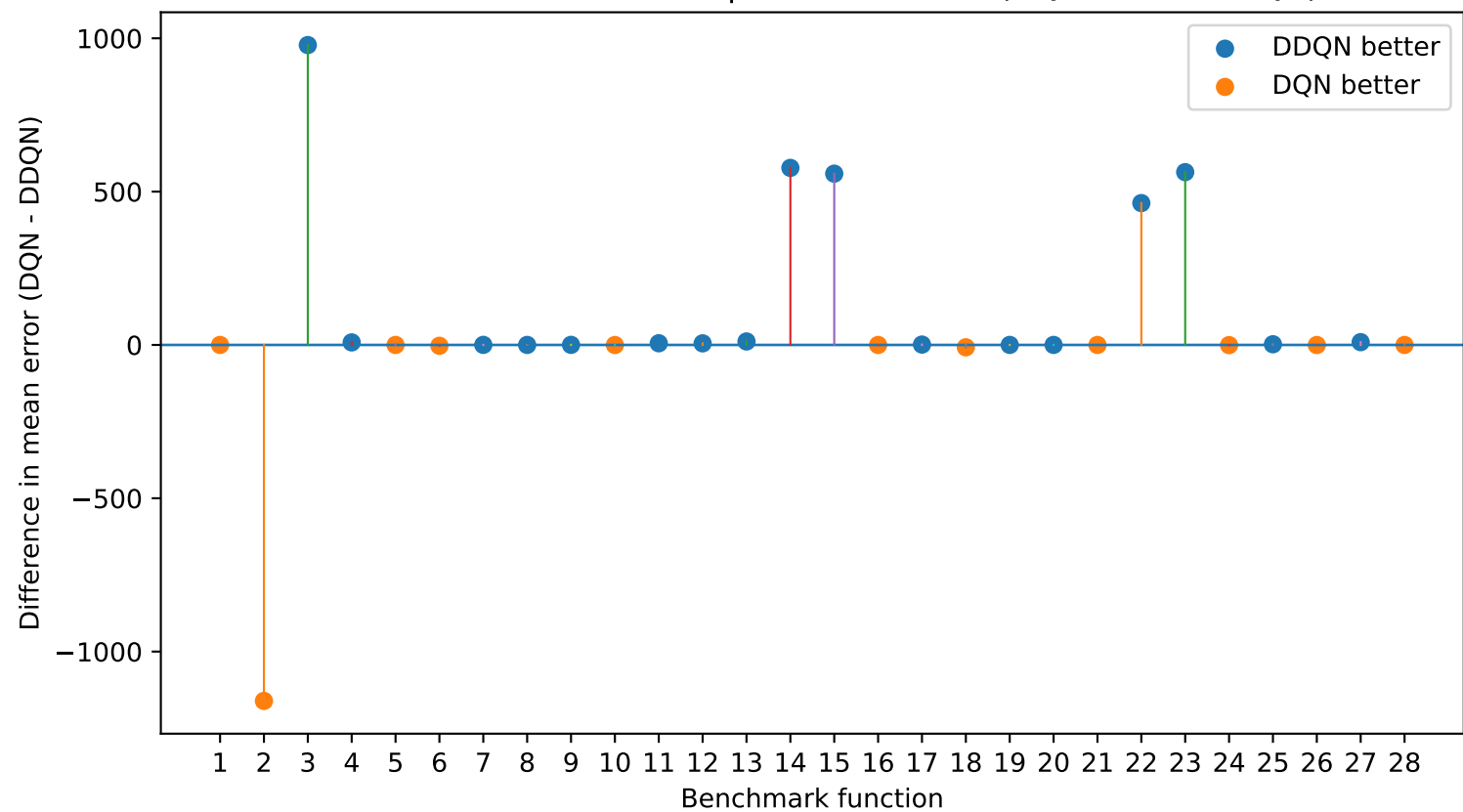
Per-function difference in optimization error (DQN - Double DQN)
