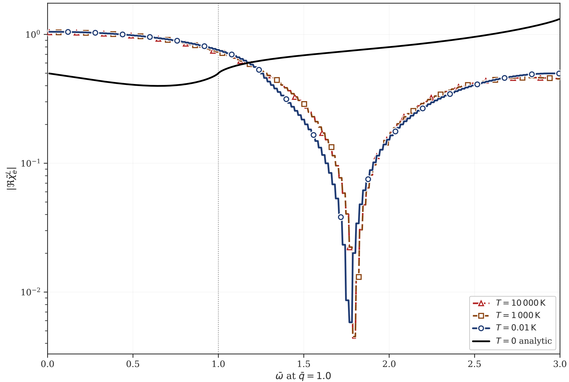
Real-part sharpening at \bar{q} = 1.0
