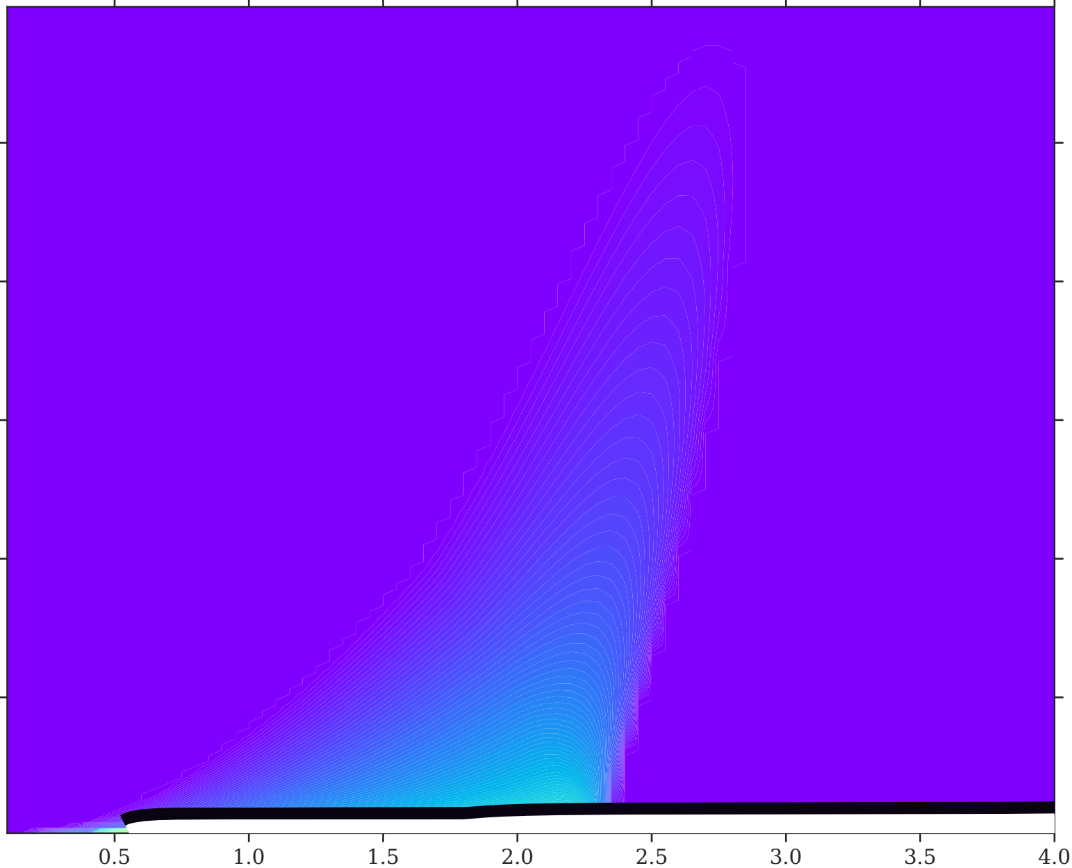
S_{ei}(q, \omega) — electron-ion cross — Contour Map
