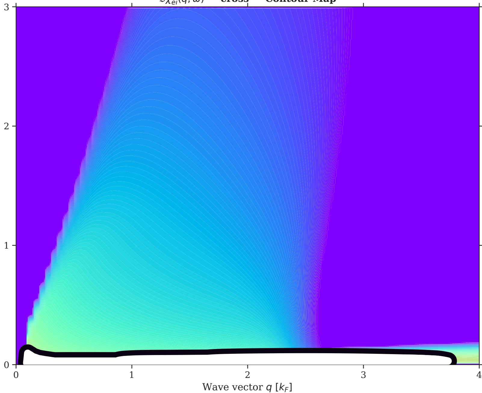
\Im \tilde{\chi}_{ei}^L(\bar{q}, \bar{\omega}) — cross — Contour Map
