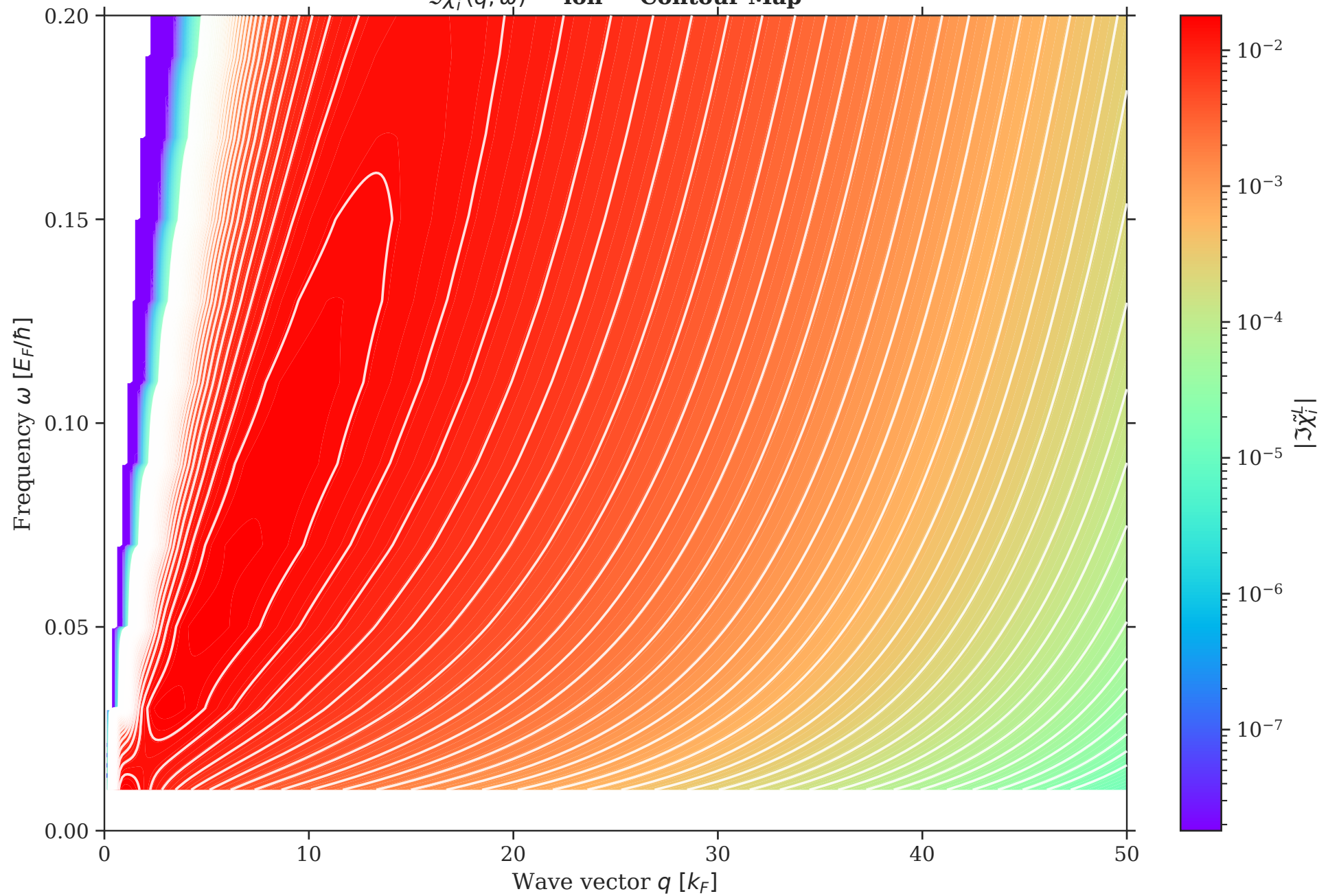
\Im \tilde{\chi}_i^L(\bar{q}, \bar{\omega}) — ion — Contour Map
