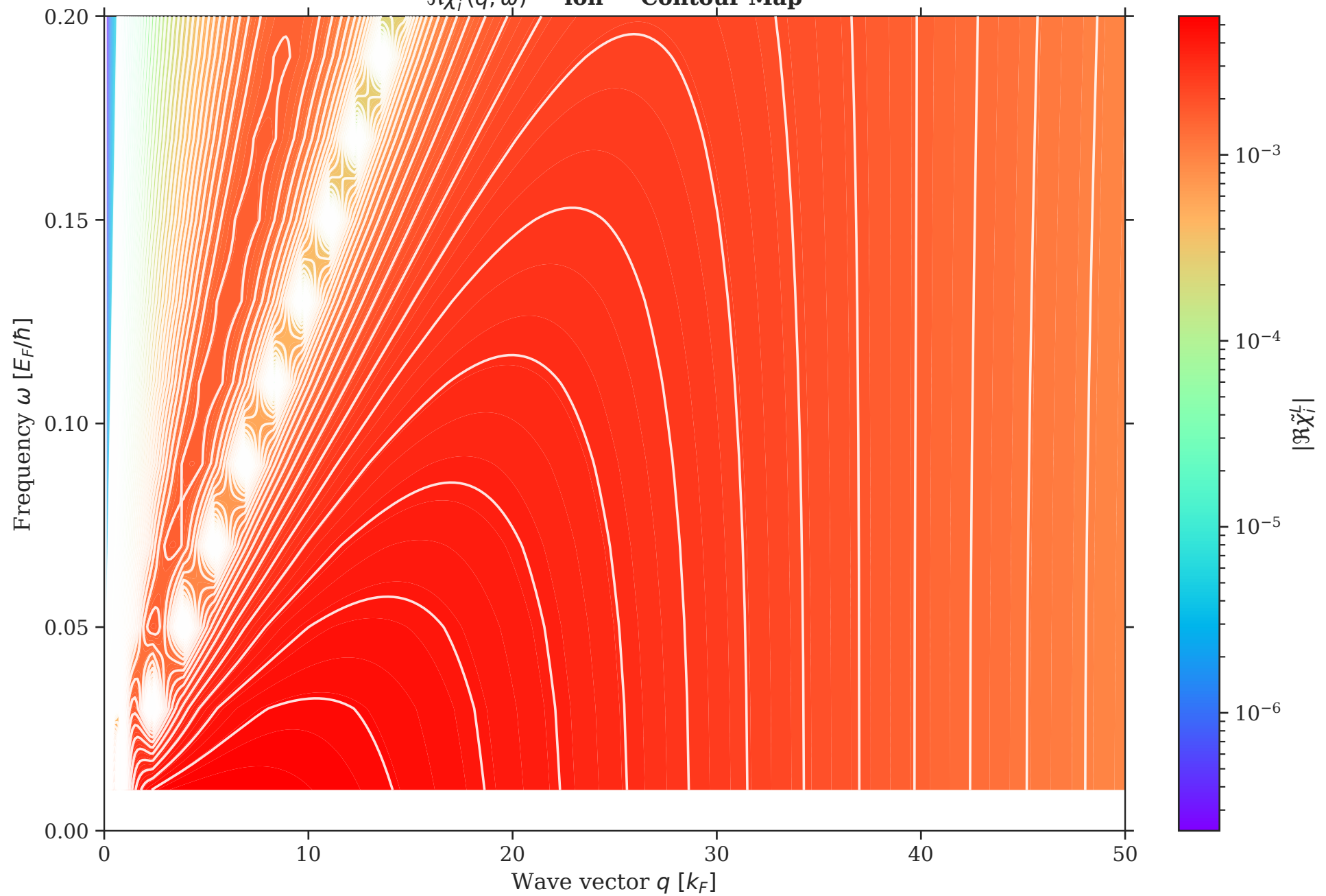
\Re\tilde{\chi}_I^L(\bar{q}, \bar{\omega}) — ion — Contour Map
