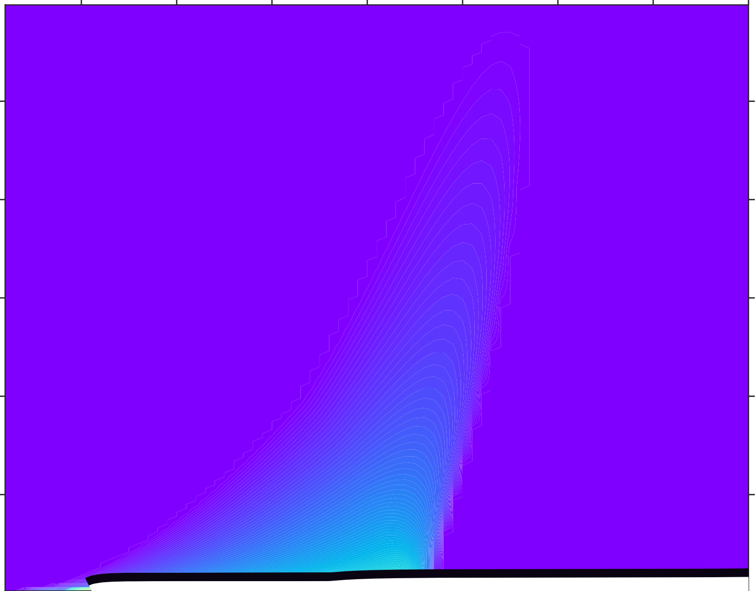
S_{ei}(q, \omega) — electron-ion cross — Contour Map
