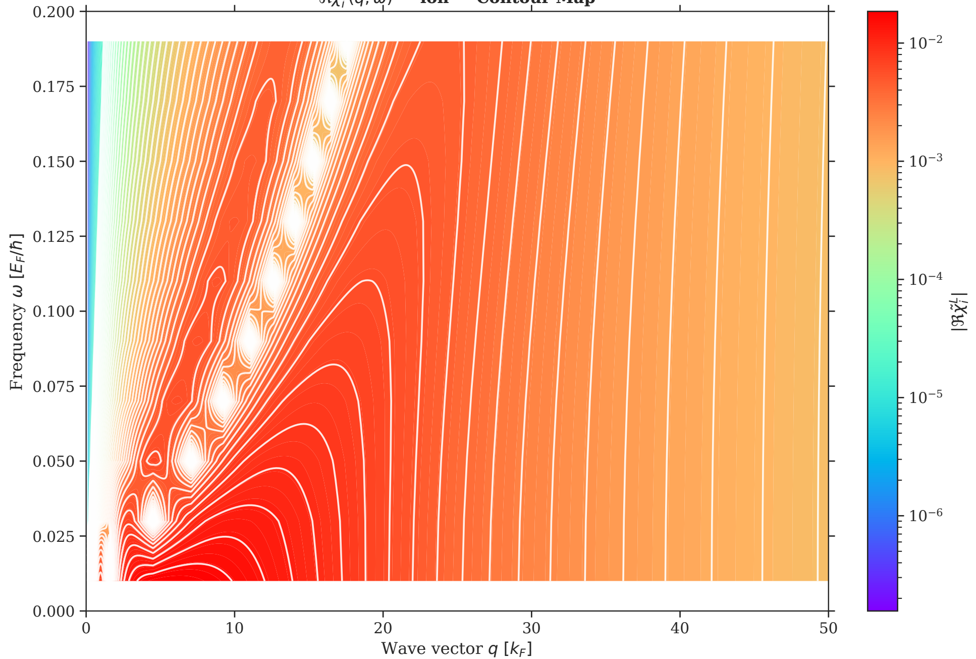
\Re\tilde{\chi}_I^L(\bar{q}, \bar{\omega}) - \text{ion} - \text{Contour Map}
