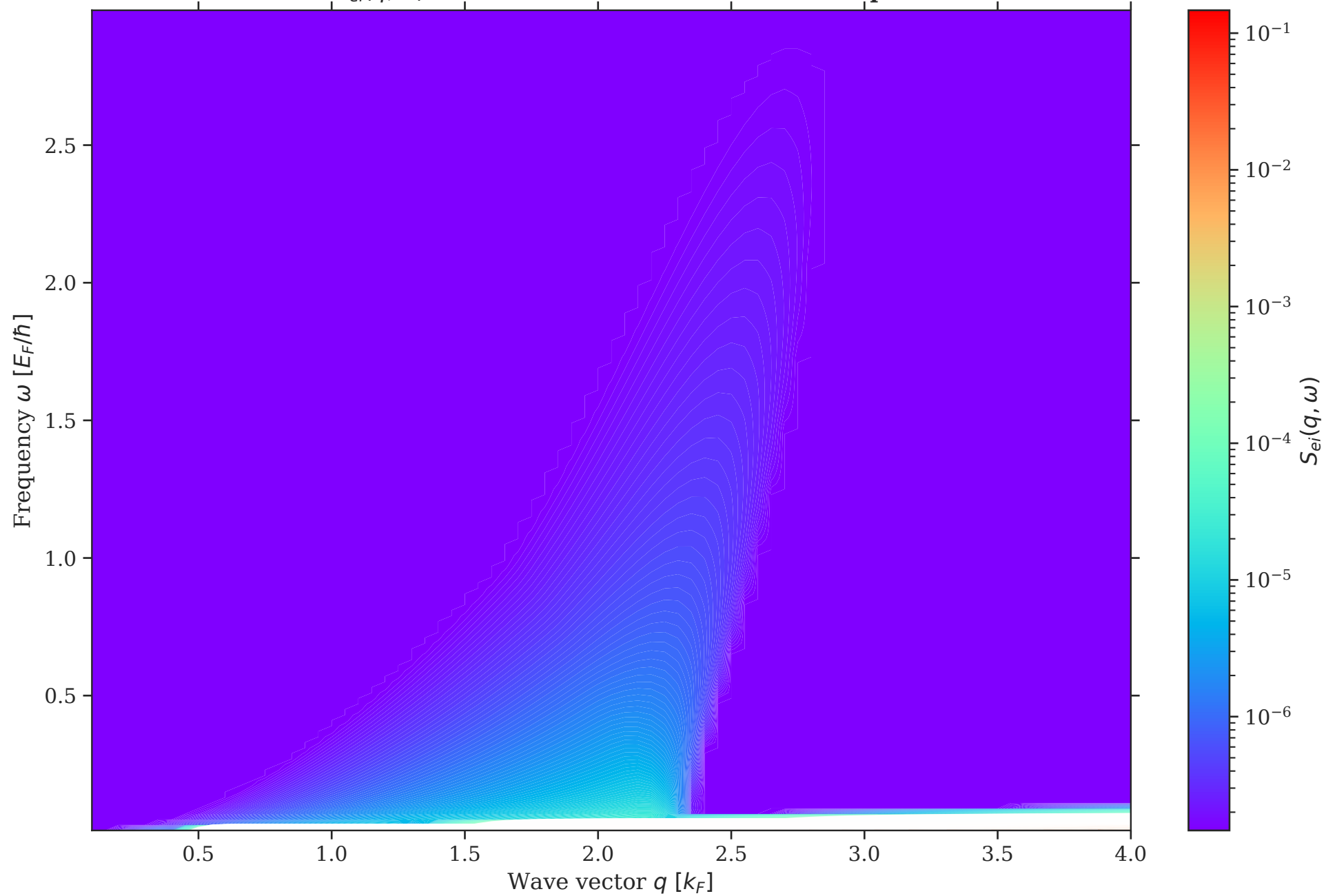
S_{ei}(q, \omega) — electron-ion cross — Contour Map
