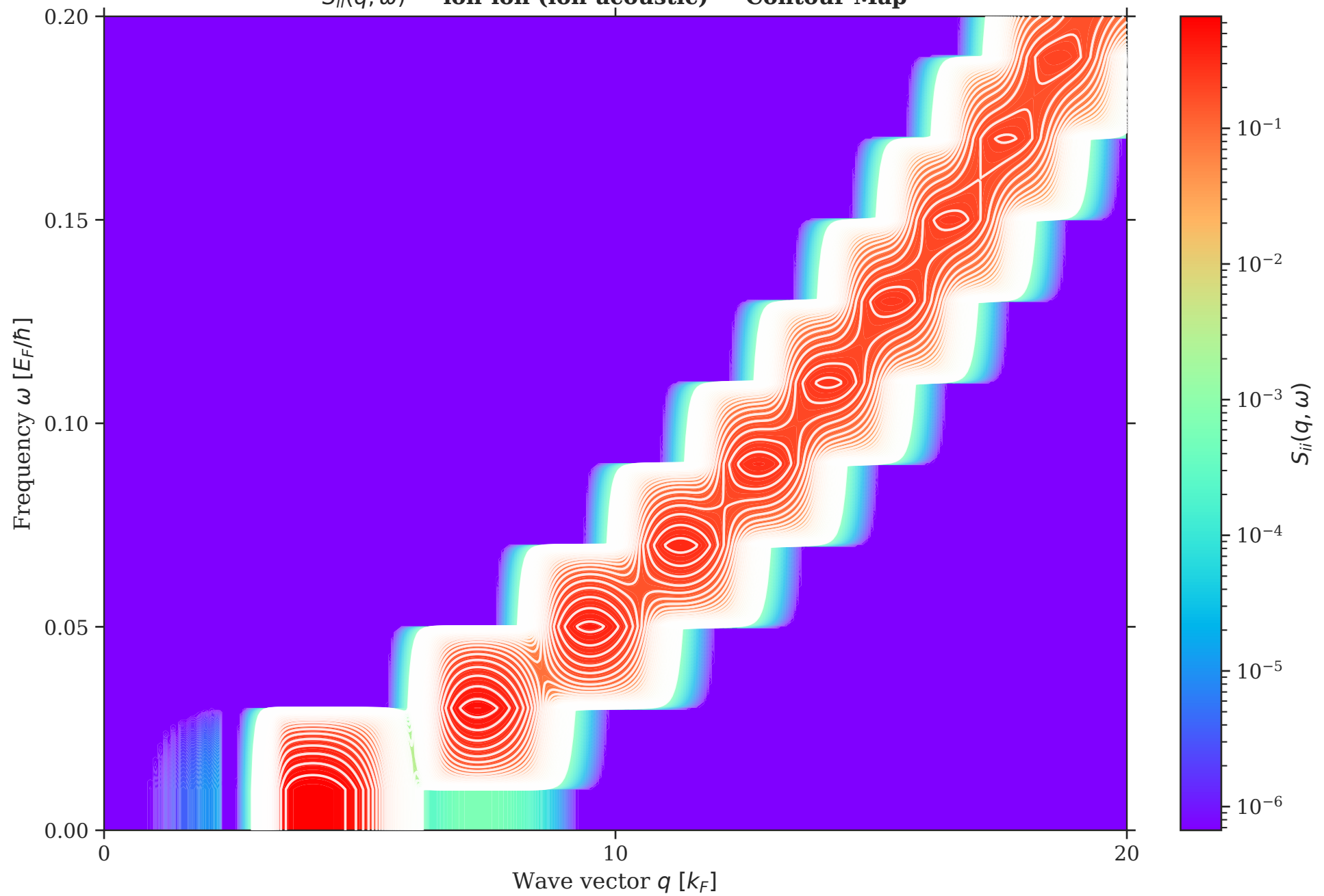
S_{ii}(q, \omega) — ion-ion (ion-acoustic) — Contour Map
