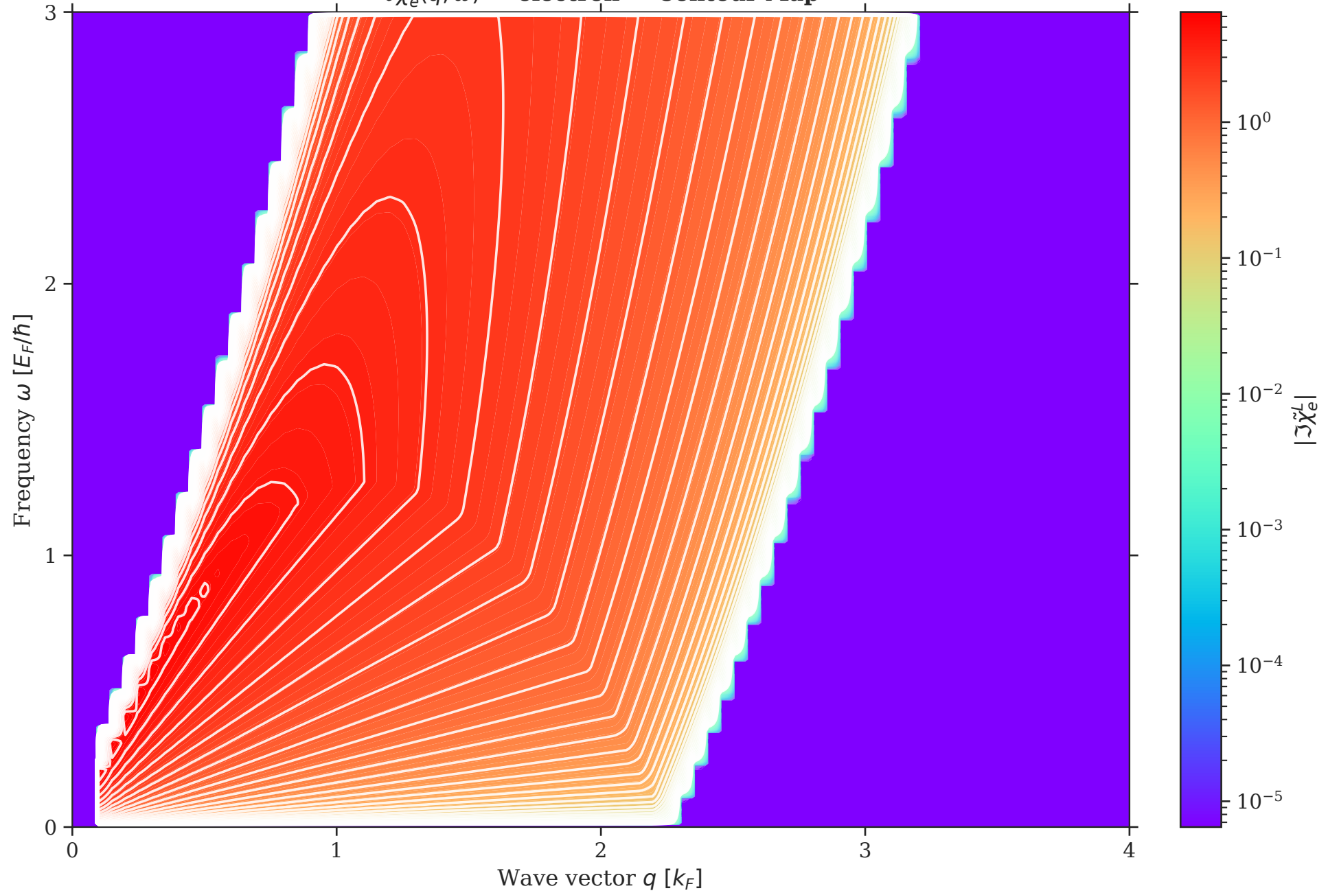
\Im\tilde{\chi}_e^L(\bar{q}, \bar{\omega}) — electron — Contour Map
