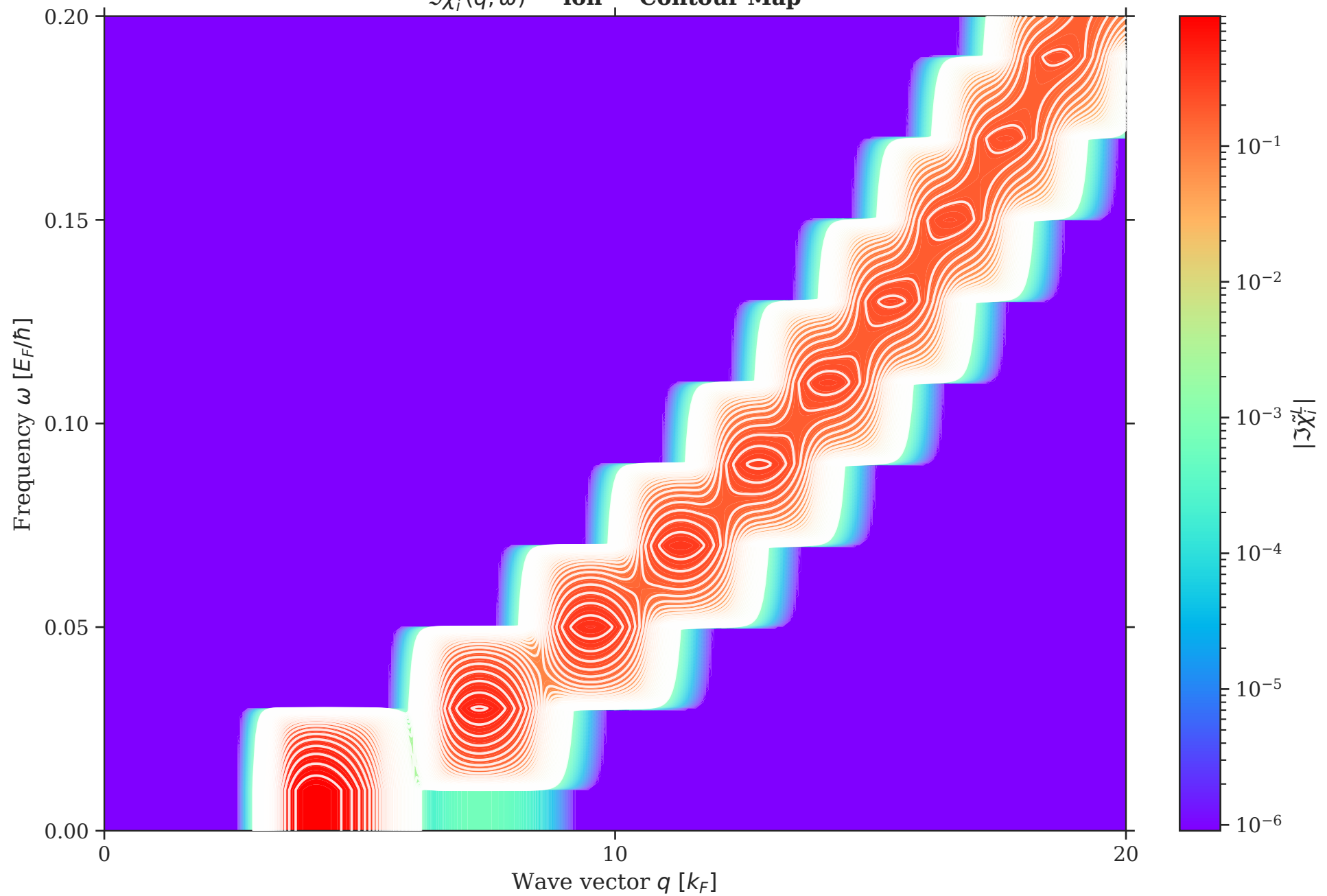
\Im \tilde{\chi}_i^L(\bar{q}, \bar{\omega}) - \text{ion} - \text{Contour Map}
