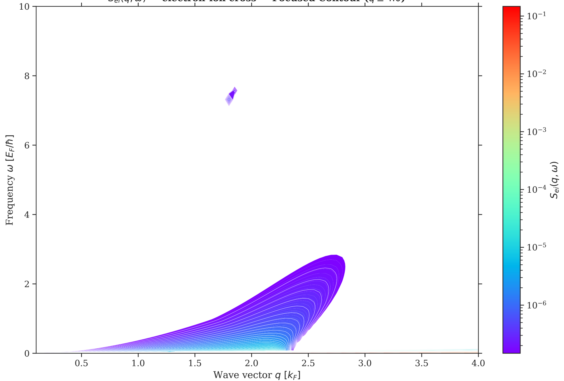
S_{ei}(q, \omega) — electron-ion cross — Focused Contour ( \bar{q} \leq 4.0 )
