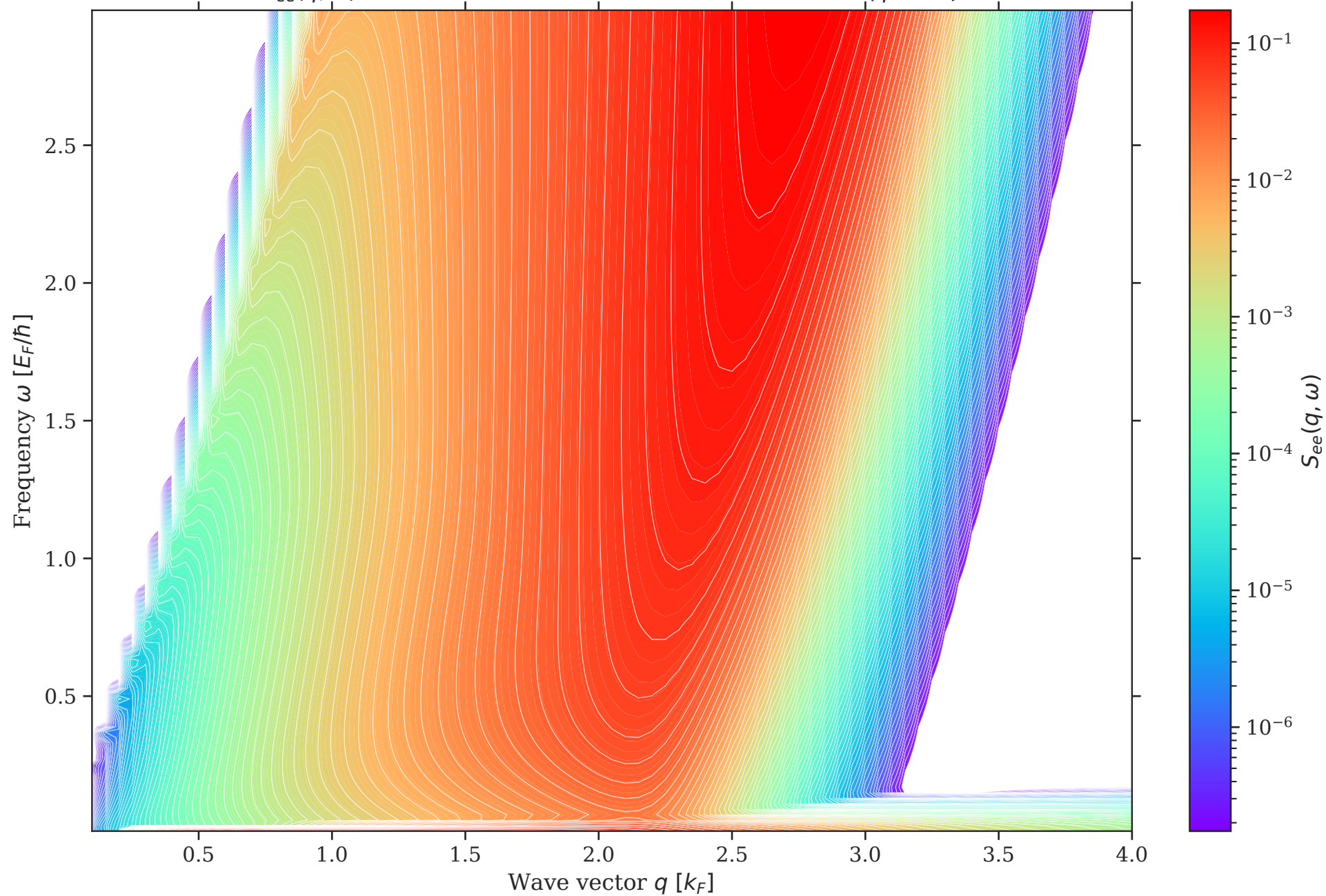
S_{ee}(q, \omega) — electron-electron — Focused Contour ( \bar{q} \leq 4.0 )
