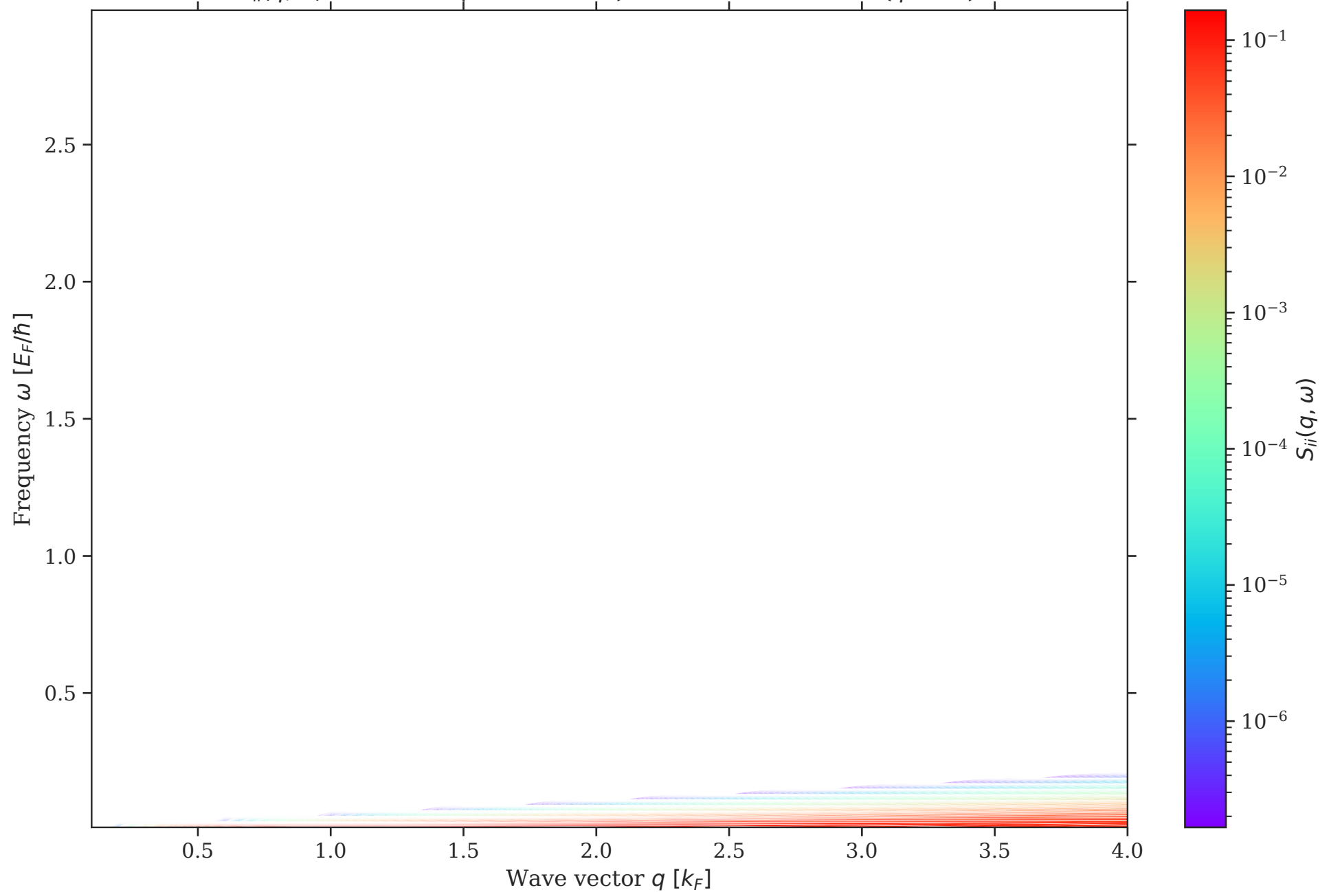
S_{ii}(q, \omega) — ion-ion (ion-acoustic) — Focused Contour ( \bar{q} \leq 4.0 )
