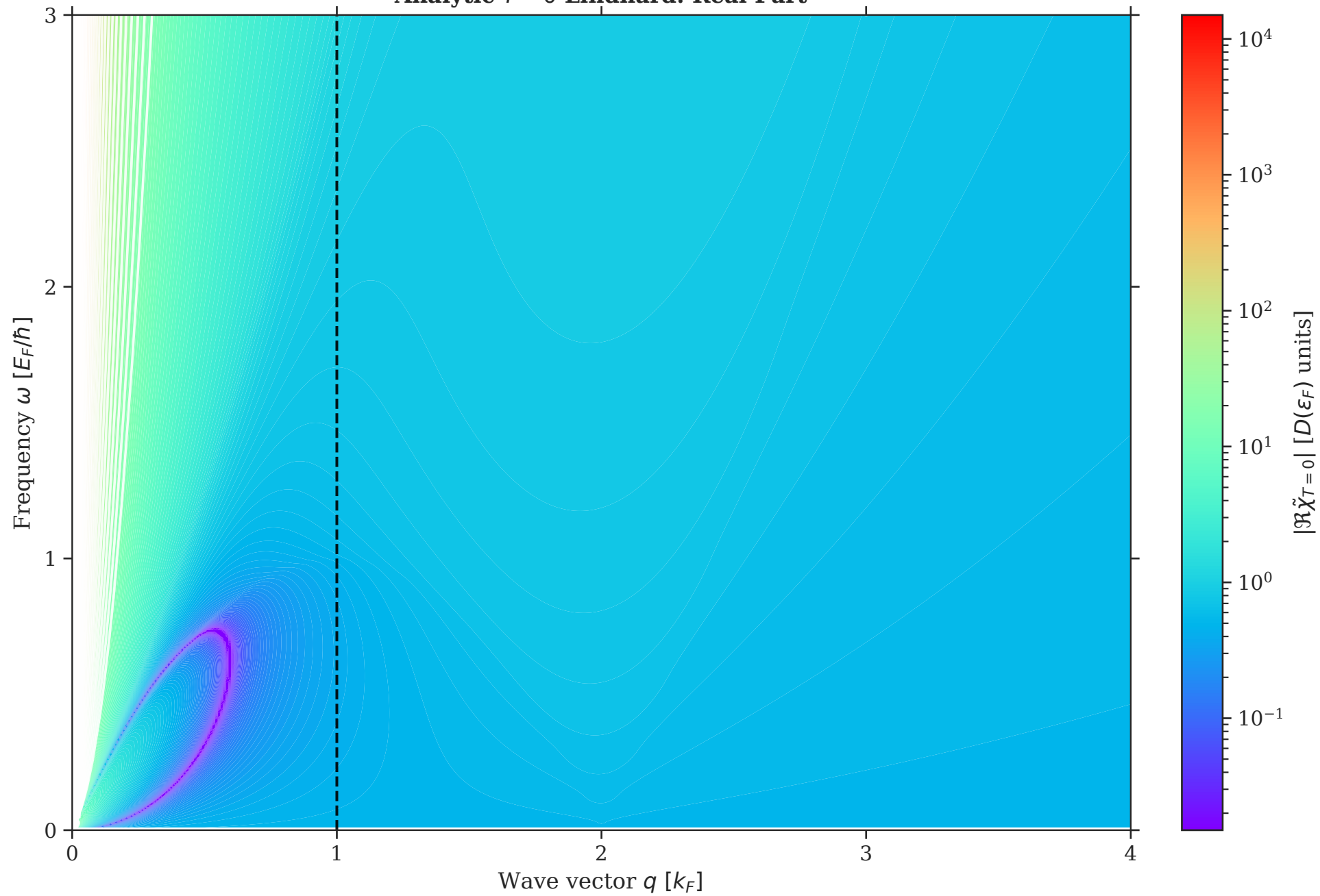
Analytic T = 0 Lindhard: Real Part
