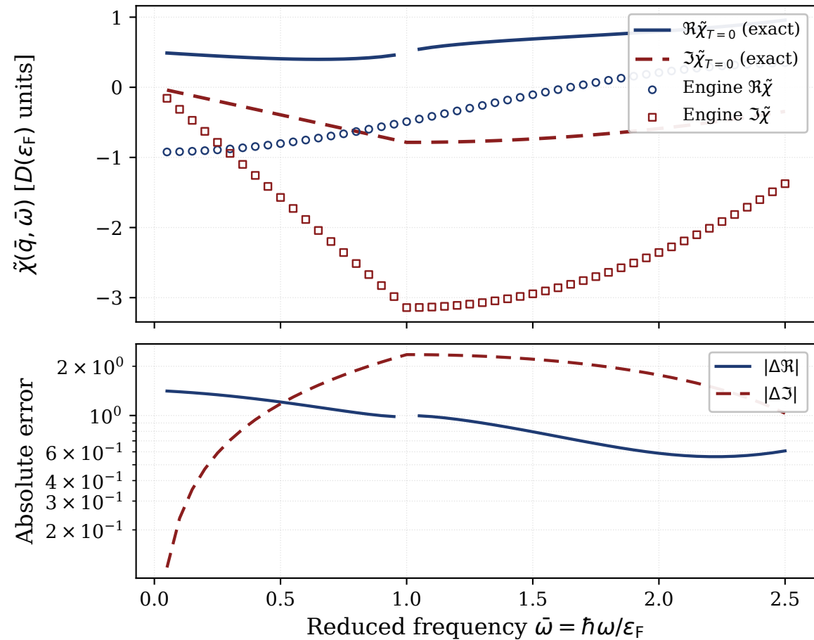
Highly degenerate limit ( r_s = 2.0 ) at \tilde{q} = 1 at T = 11 K
