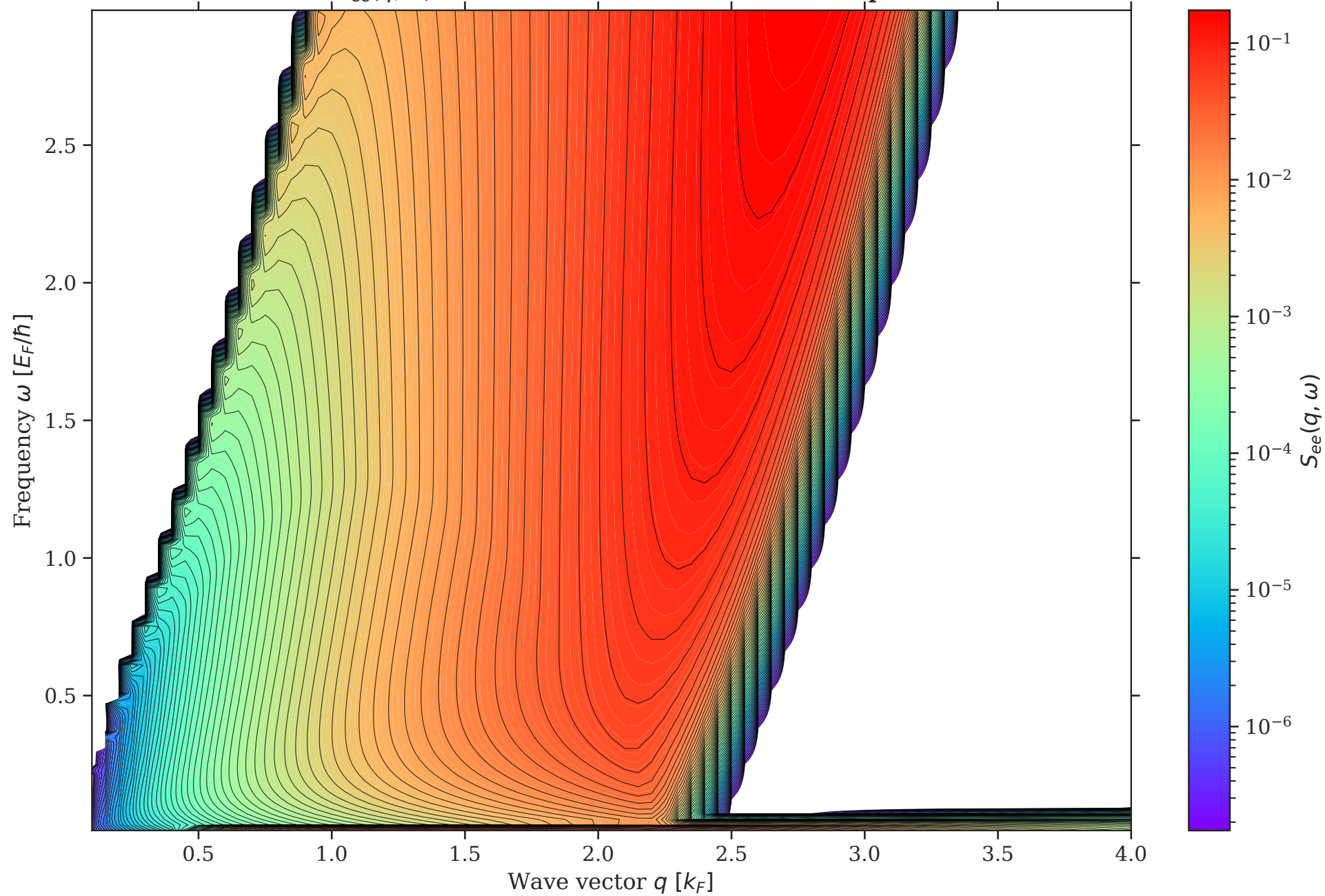
S_{ee}(q, \omega) — electron-electron — Contour Map
