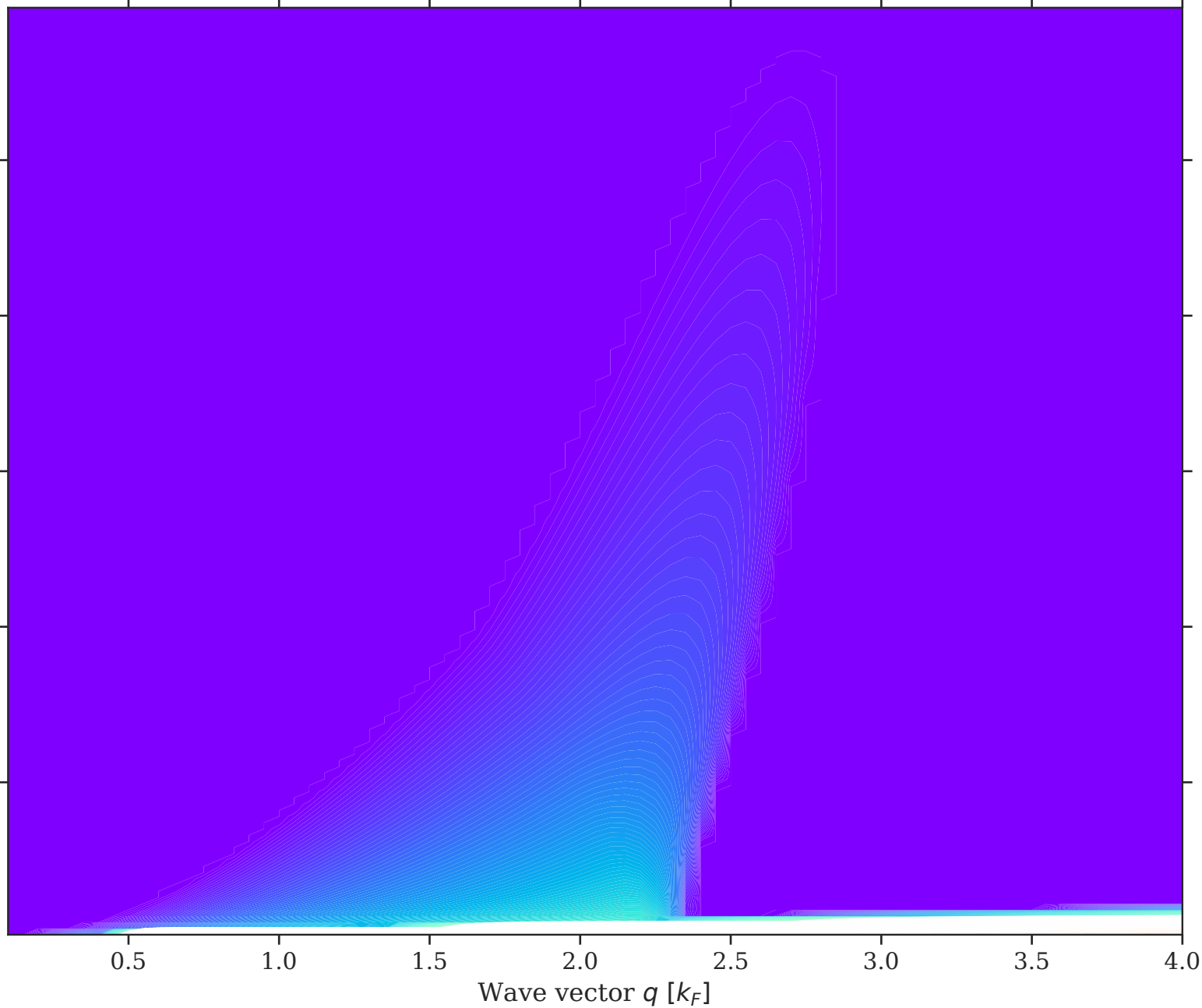
S_{ei}(q, \omega) — electron-ion cross — Contour Map
