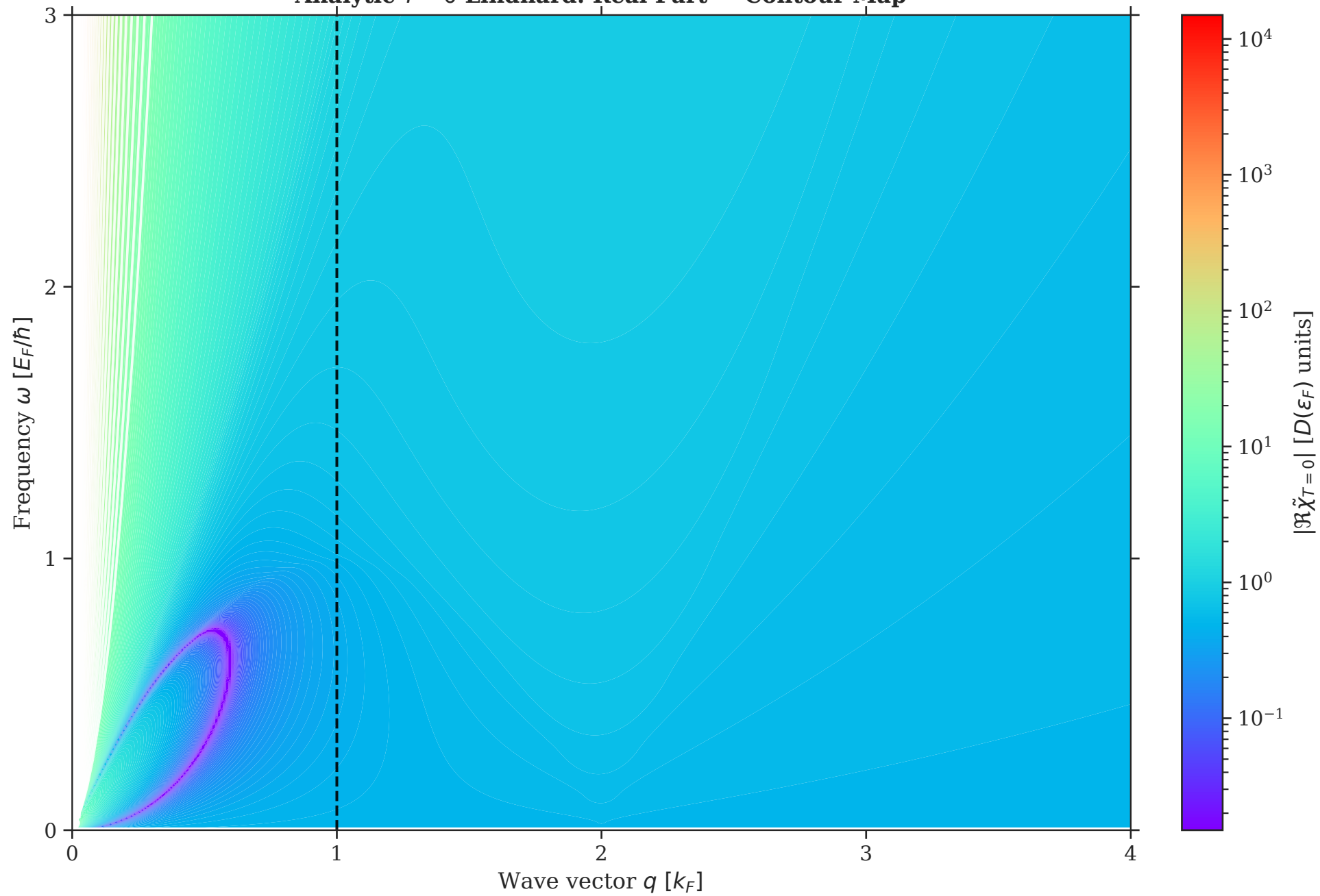
Analytic T = 0 Lindhard: Real Part — Contour Map
