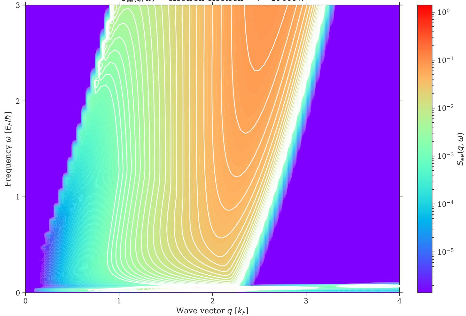
S_{ee}(q, \omega) — electron-electron — T = 10\,000\text{ K}
