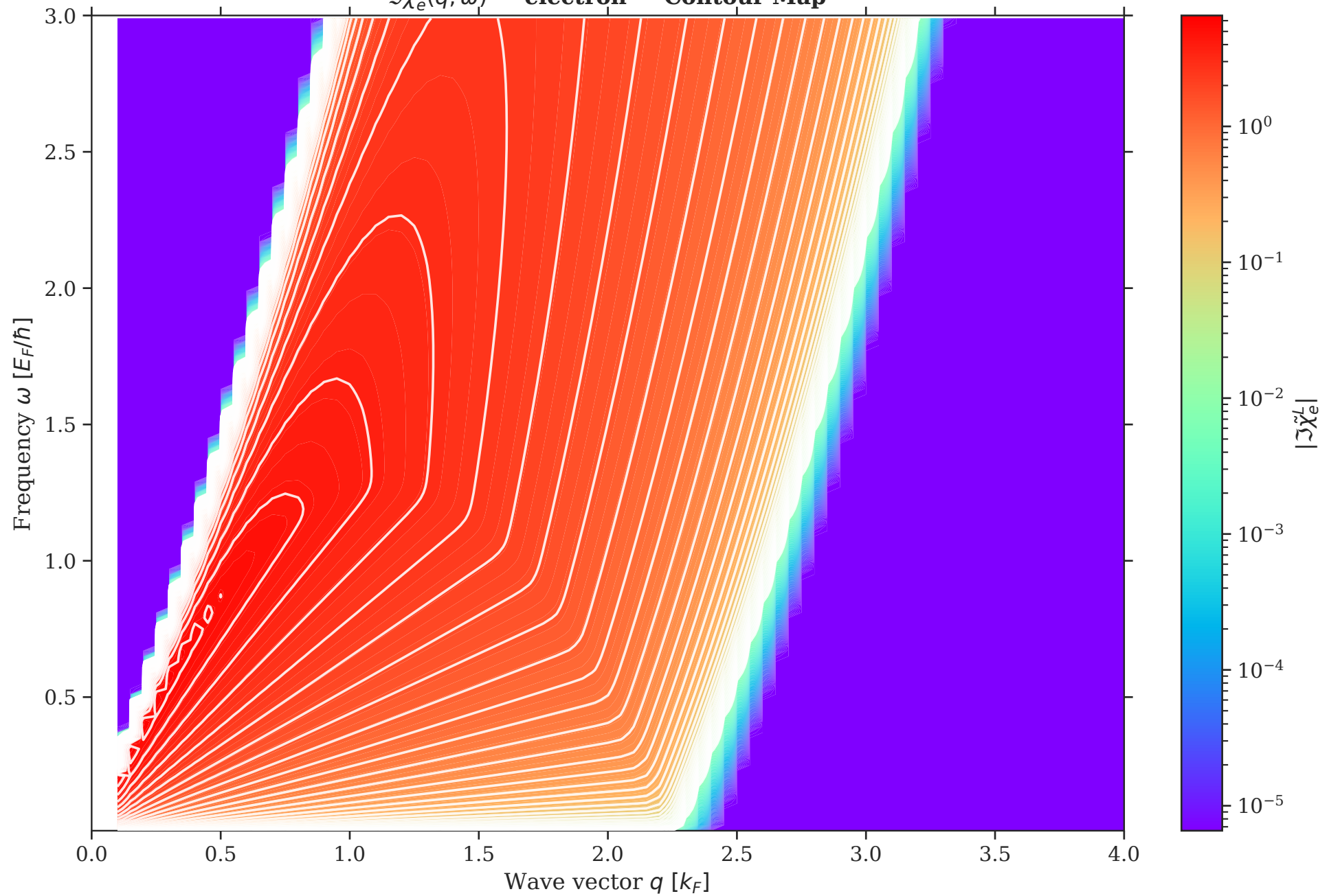
\Im \tilde{\chi}_e^L(\vec{q}, \bar{\omega}) — electron — Contour Map
