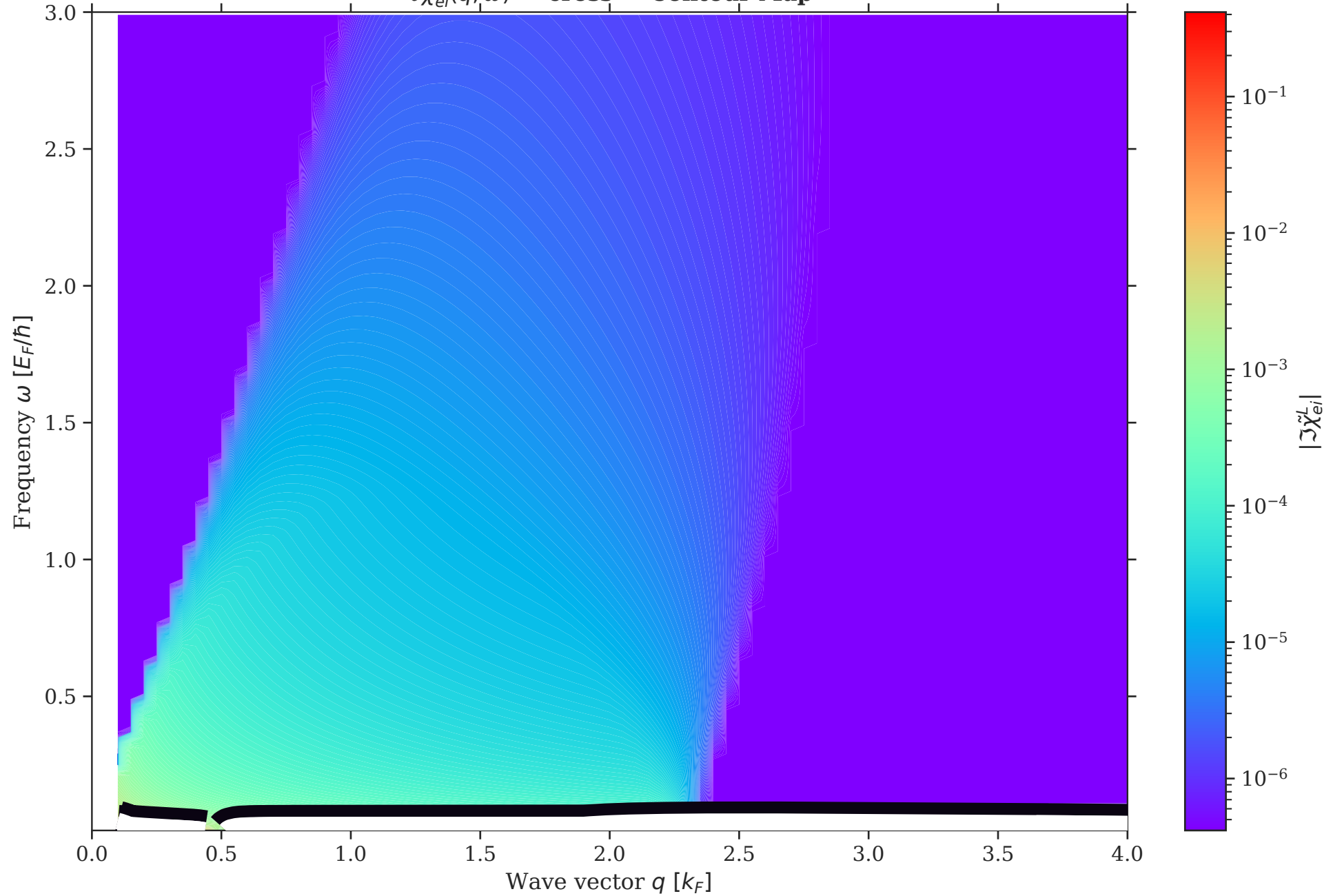
\Im \tilde{\chi}_{ei}^L(\vec{q}, \vec{\omega}) — cross — Contour Map
