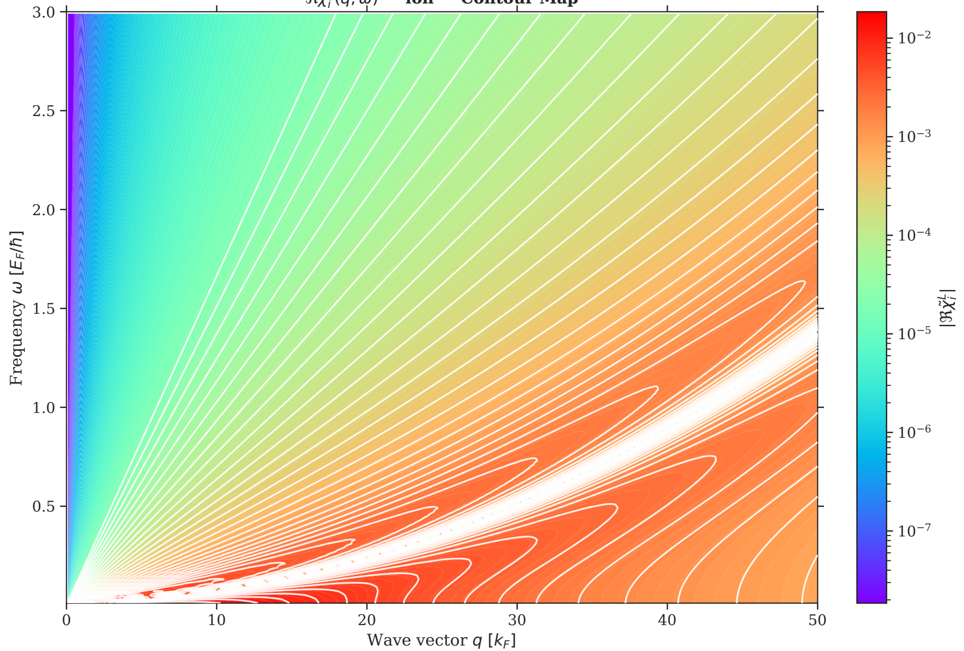
\Re\tilde{\chi}_I^L(\vec{q}, \vec{\omega}) - \text{ion} - \text{Contour Map}
