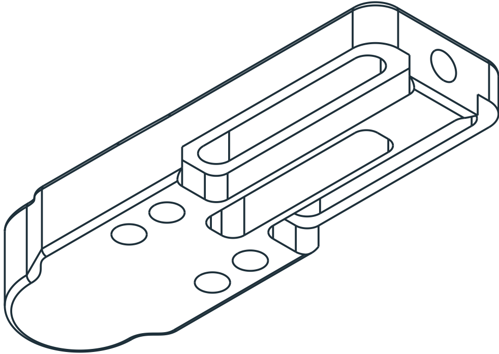
UNDERSIDE ISOMETRIC
