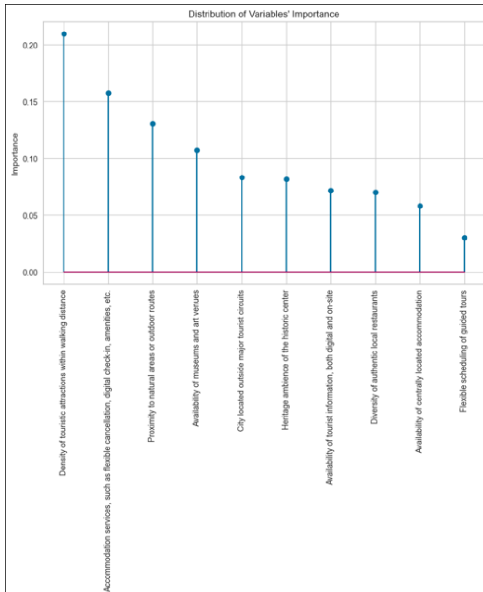
Figure 5.14: Variable Importance in Random Forest Model. Source: Author's own elaboration.
