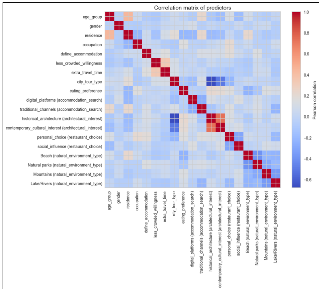
Figure 5.15: Correlation Heatmap . Source: Author's own elaboration.
