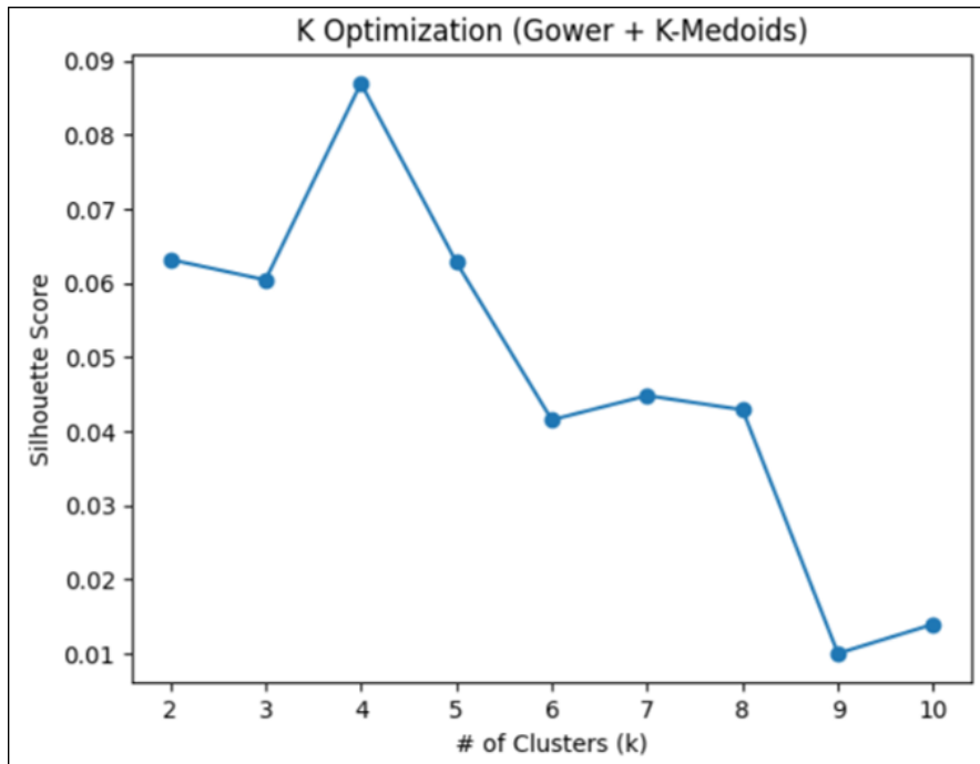
Figure 3.21: Silhouette Scores and Plot. Source: Author's own elaboration.
