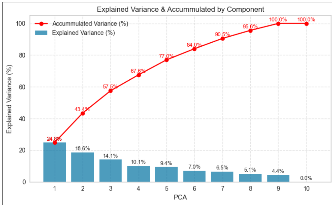
Figure 3.23: Cumulative Explained Variance (PCA) . Source: Author's own elaboration.
