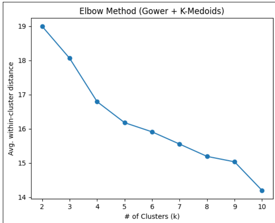
Figure 3.20: Elbow plot. Source: Author's own elaboration.
