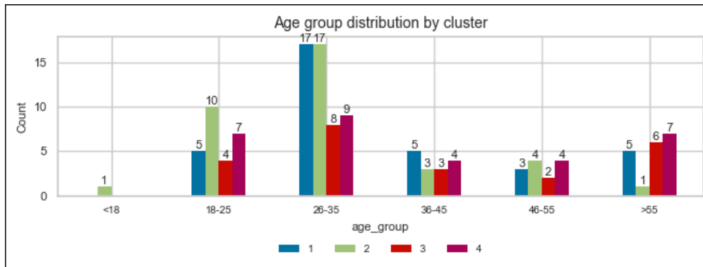
Figure 4.22: Age Range by Cluster. Source: Author's own elaboration.
