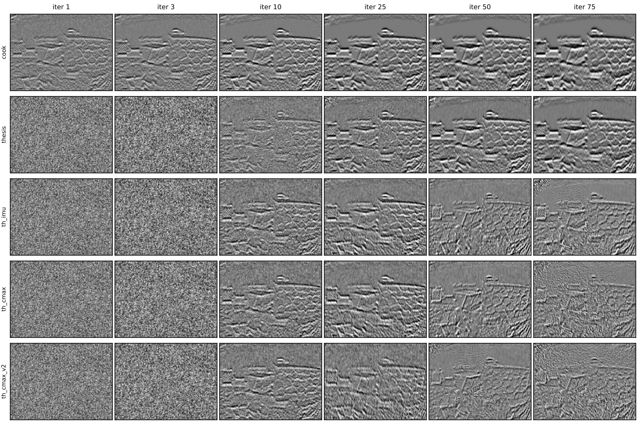
boxes seg_B: intensity map across message-passing iterations (frame 40)
