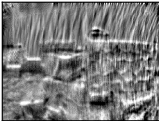
|r| = 0.35
