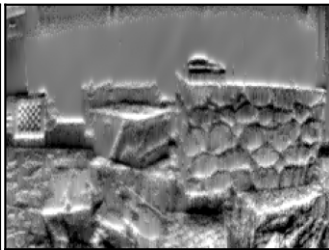
|r| = 0.48
