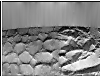
|r| = 0.67
