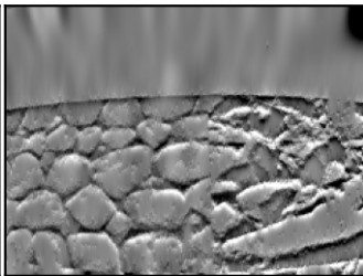
|r| = 0.42
