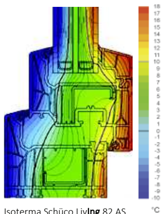
Isotherma Schüco LivIng 82 AS Isothermal flow in Schüco LivIng 82 AS
