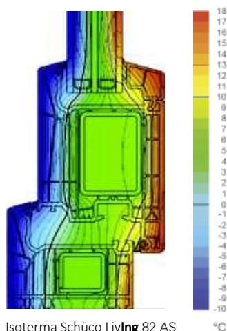
Isotherma Schüco LivIng 82 AS con anta portoncino Isothermal flow in Schüco LivIng 82 AS with entrance door leaf
