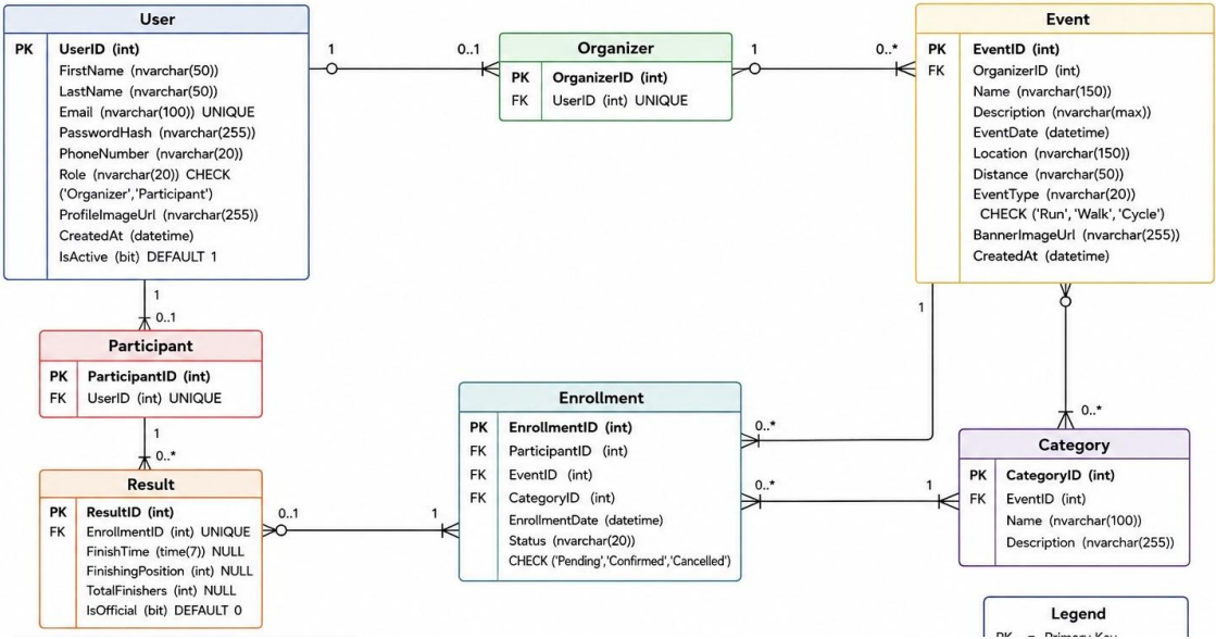
Race Day – Entity Relationship Diagram (ERD)
