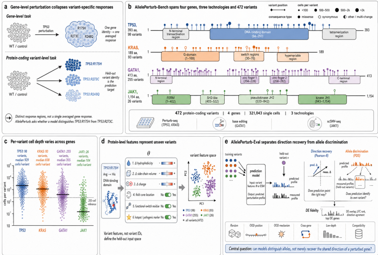
Figure 1: AllelePerturb defines perturbation prediction at protein-coding variant resolution. a , Conceptual distinction between gene-level and protein-coding variant-level perturbation prediction. Gene-level perturbation identity collapses responses from different variants of the same gene into a single averaged effect, whereas AllelePerturb treats a held-out protein-coding variant as the prediction target and asks whether models can distinguish allele-specific responses within the same gene. b , Overview of AllelePerturb-Bench. The benchmark integrates 472 protein-coding variants across four genes and protein architectures (TP53, KRAS, GATA1 and JAK1), spanning three experimental technologies: Perturb-seq, base editing and scSNV-seq. c , Per-variant cell depth varies substantially across genes, providing a range of sampling regimes for evaluation (98, 93, 255 and 26 variants; 83.4k, 83.6k, 149.2k and 4.9k cells for TP53, KRAS, GATA1 and JAK1, respectively). d , Each variant is represented by a 6-dimensional biophysical vector \theta encoding changes in hydrophobicity, side-chain volume and charge, together with fold-core location, functional-switch residue status and hotspot/pathogenic annotation. e , AllelePerturb-Eval separates prediction quality into direction recovery (Pearson- \delta ), allele-level discrimination (PDS) and differential-expression fidelity, and defines six split strategies to test random generalization, positional extrapolation, mechanistic extrapolation, cross-gene transfer, low-depth evaluation and compatibility with existing protocols.
