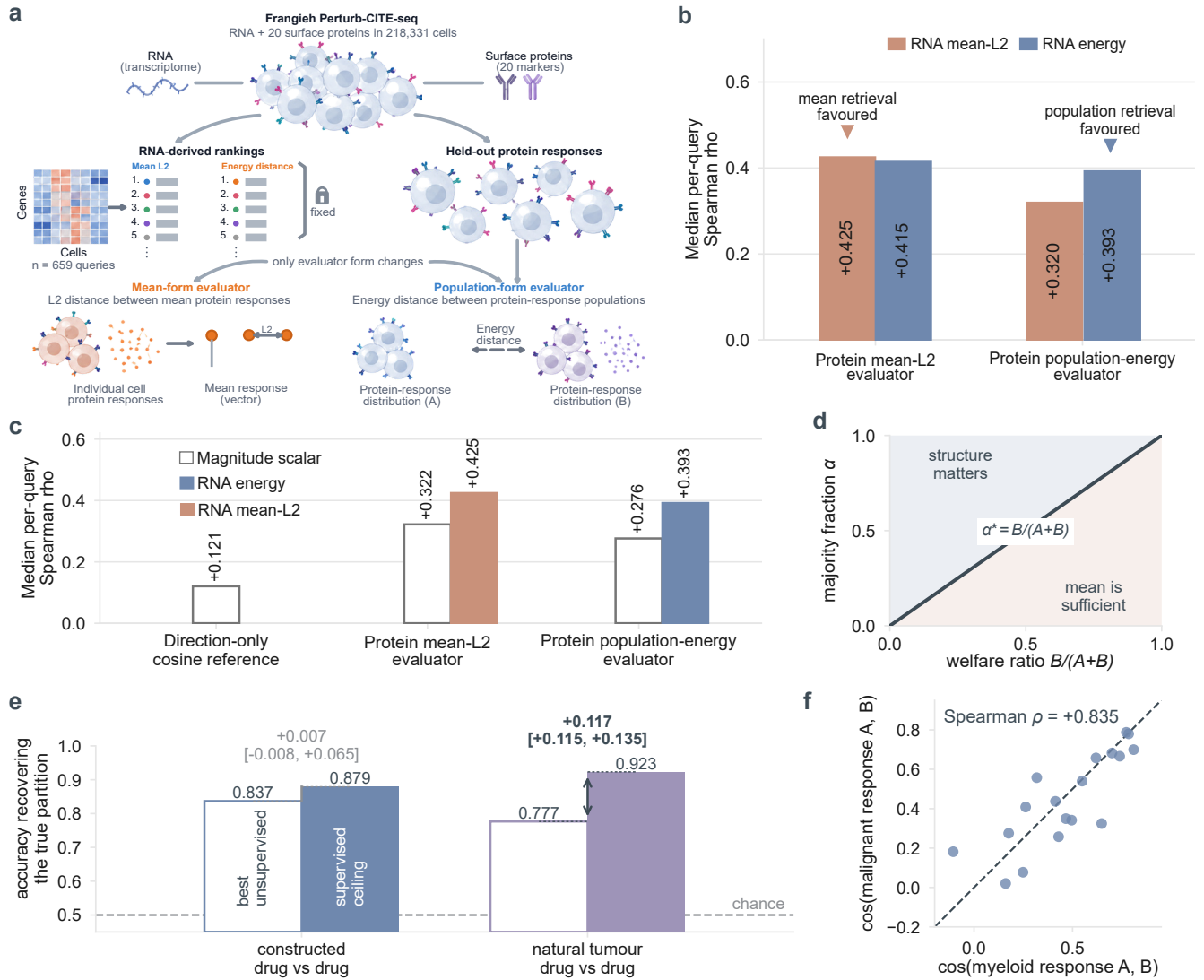
Figure 4: External evaluator form reverses the preferred retrieval strategy under matched geometry, whereas heterogeneity need not reorder candidates. a–c , The same fixed RNA-derived rankings evaluated using held-out protein responses from Frangieh Perturb-CITE-seq. a , RNA and 20 surface proteins are measured in the same 218,331 cells; protein measurements are unavailable to the retrieval methods. Two primary protein evaluators are constructed from the same cells: a magnitude-aware mean evaluator using negative Euclidean distance between control-referenced mean protein responses, and a population evaluator using negative energy distance between protein-response populations. b , Median per-query Spearman correlation across n = 659 queries for magnitude-aware mean-L2 and population-energy RNA retrieval. Under the protein mean-L2 evaluator, RNA mean-L2 and RNA energy reach +0.4255 and +0.4150, respectively, with a median paired difference of -0.0208 (energy minus mean-L2). Under the protein population-energy evaluator, the ordering reverses: +0.3199 and +0.3930, with a median paired difference of +0.0538. The paired difference has the same sign in Co-culture ( -0.0105 , +0.0466), Control ( -0.0363 , +0.1342) and IFN \gamma ( -0.0318 , +0.0384) for the mean and population evaluators, respectively. c , A scalar RNA response-magnitude ranking reaches +0.3223 and +0.2764 under the protein mean-L2 and population-energy evaluators, respectively; its value under the direction-only protein-cosine reference is +0.1206. d , HIR-Bench boundary \alpha^* = B/(A+B) separating settings in which the mean is sufficient from those in which subpopulation structure can change the preferred candidate. e , f , Four glioblastoma tumours analysed in disjoint malignant and myeloid compartments with matched drugs and controls. e , Recovery of within-patient drug-response identity; open bars, best unsupervised method; filled bars, supervised probe. Median paired gap, +0.117 (95% patient-level cluster-bootstrap CI +0.115 to +0.135, n = 36 splits), versus +0.007 in the constructed comparator. f , Myeloid-response similarity versus malignant-response similarity across compartments (Spearman \rho = +0.835 , n = 18 drug pairs); dashed line, equal similarity.
