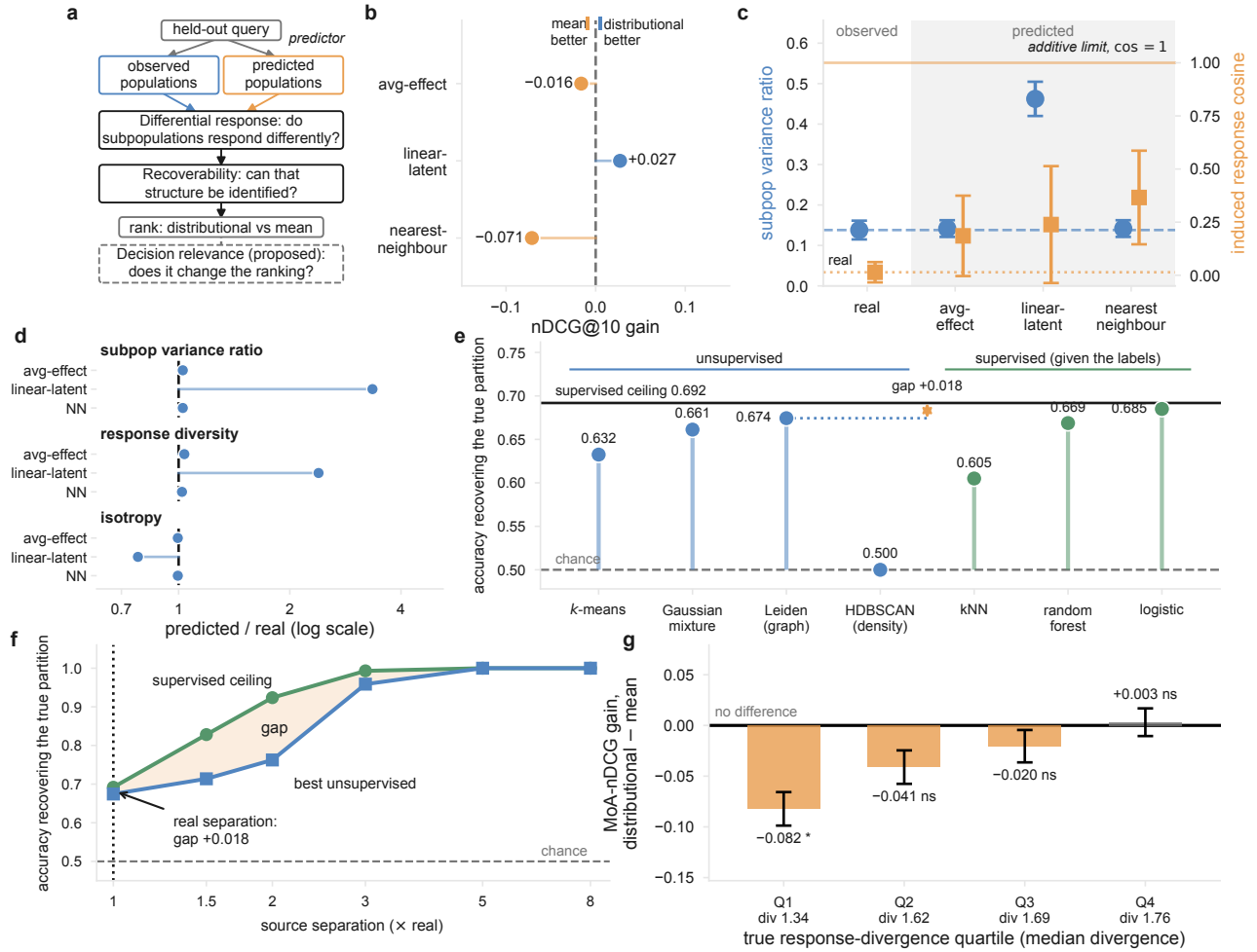
Figure 5: When can population-level information improve drug retrieval? a , Three requirements connect cellular heterogeneity to a change in candidate ranking. Differential response and recoverability are measured directly in this study; decision relevance is a downstream requirement proposed from the combined results and is shown separately. b , When candidate populations are generated by perturbation predictors rather than directly observed, the population-level advantage is small and inconsistent across the three predictor families tested (distributional minus mean nDCG@10: -0.071, -0.016 and +0.027). c , Differential response. Predicted populations can preserve heterogeneity in the starting cell population while failing to reproduce state-specific perturbation effects; additive predictors necessarily assign the same perturbation response to every cellular state. d , Structure diagnostics of predicted candidate populations relative to the real population they replace, on a ratio axis with the reference at 1. The additive average-effect and nearest-neighbour predictors reproduce subpopulation variance, response diversity and isotropy almost exactly (ratios 0.99–1.04); the linear-latent model overshoots the first two (3.35 and 2.39) and reduces isotropy (0.78). e , Recoverability in a controlled two-state mixture. The best unsupervised method reaches 0.674 against a supervised ceiling of 0.692; the low ceiling is partly explained by pooling multiple drugs into broad classes, whereas individual drug pairs reach a ceiling of 0.879. Natural tumour tissue shows a larger supervised–unsupervised gap (Fig. 4d). f , Increasing the separation of the constructed states pulls the supervised ceiling away from unsupervised recovery, confirming that the probe can detect additional recoverable information when it is present. Shading marks the region unsupervised clustering cannot reach. g , Decision relevance is not implied by differential response alone. Mechanism-of-action gain does not become a significant positive advantage in the highest response-divergence quartile (mean +0.003, q = 0.57 ), whereas the lowest-divergence quartile is significantly negative. Asterisk, q < 0.05 after Benjamini–Hochberg correction; ns, not significant.
