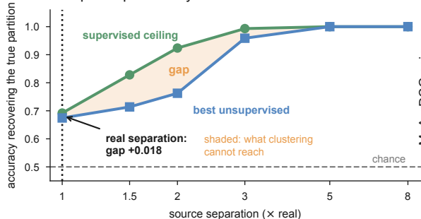
f The probe pulls away when structure is there
