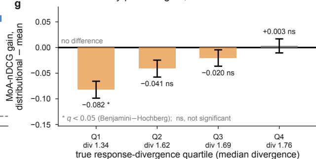
g Where theory predicts gain, there is none
