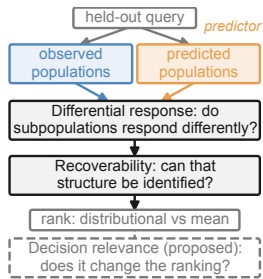
a Predict-then-rank, and three conditions
