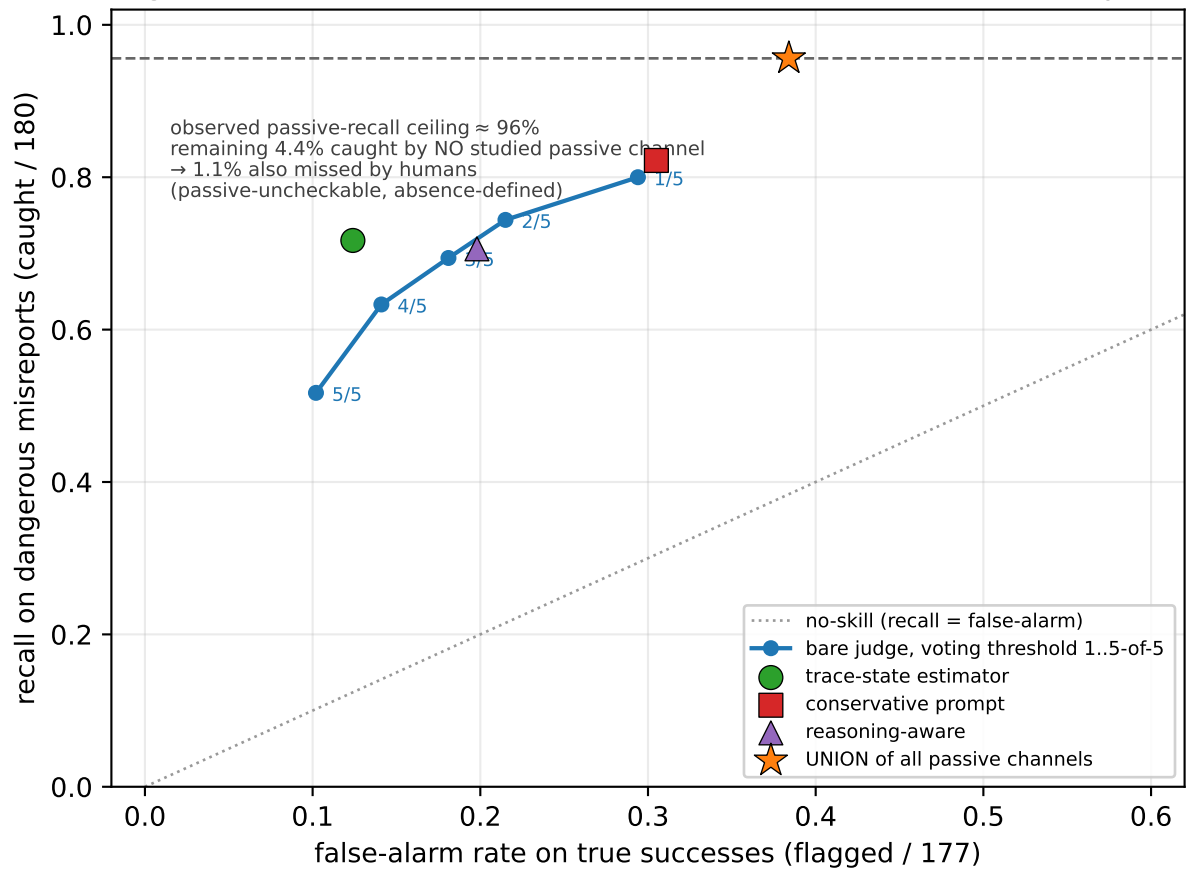
Passive auditing: a recall-false-alarm frontier (observed under the studied passive channels)
