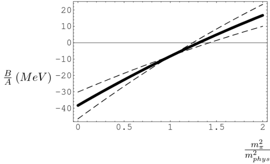
Figure 25: Binding Energy per nucleon as a function of the pion mass for the O^{16} atom. Figure taken from [11]
