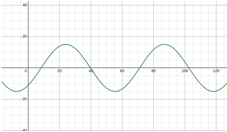
Figure 16: Initial position of a plane wave
