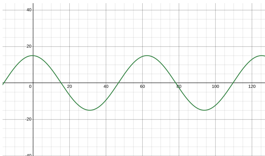
Figure 17: The plane wave at a later time, has moved to the right
